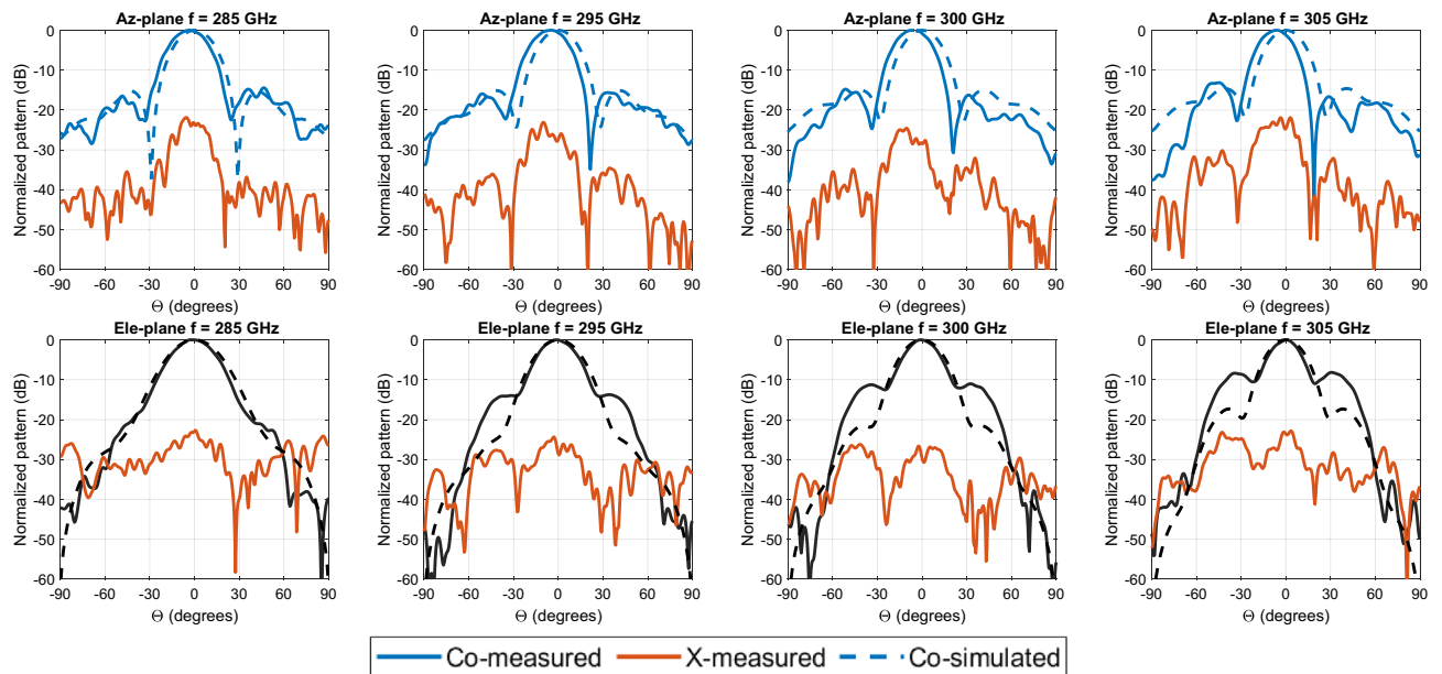
Figure 8. Measured (solid lines) and simulated (dashed lines) normalized radiation patterns of the proposed antenna of the azimuth (Az.) and elevation (Ele.) planes at different frequencies.
