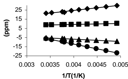
Figure 3. Temperature dependence of selected ^1\text{H} NMR resonances of complex 6 .
