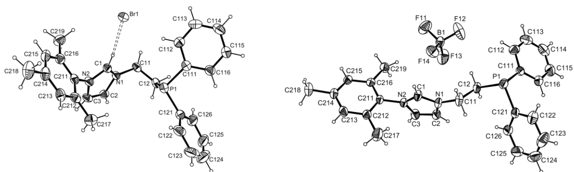
Figure 1. An ORTEP view of compounds 1a (left) and 1b (right). Ellipsoids are drawn at the 50% probability level. For 1a , C-H...Br bonding interaction is shown as dashed line.
