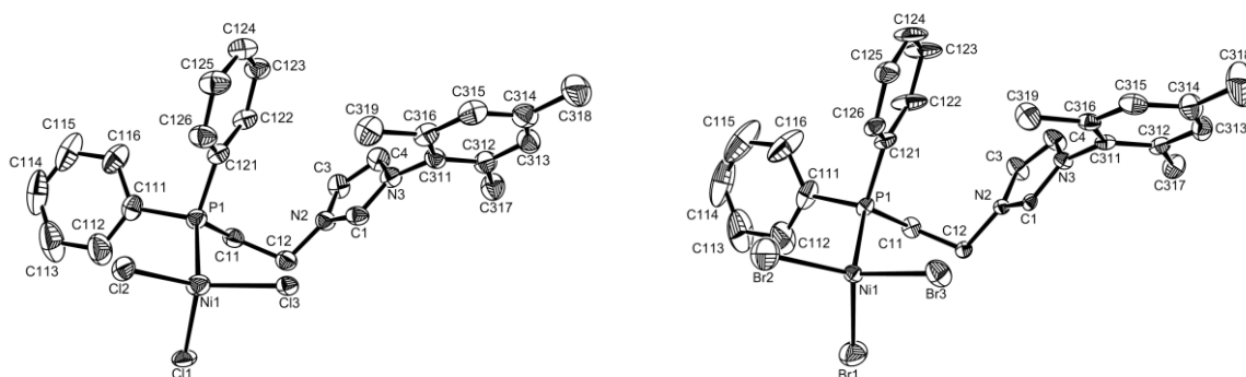
Figure 2. An ORTEP view of compounds 6 (left) and 7 (right). Ellipsoids are drawn at the 50% probability level. H atoms have been omitted for clarity.
