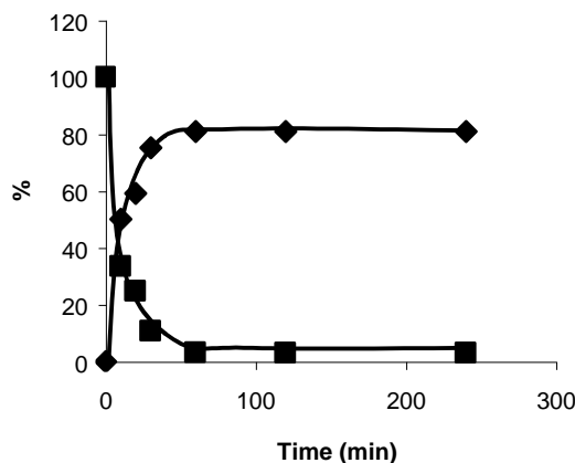
Figure 5. Percent conversion of 4-chloroanisole 8 (■) vs time to give coupling product 10 (◆, GC yield). Conditions are as shown in Experimental (method A).
