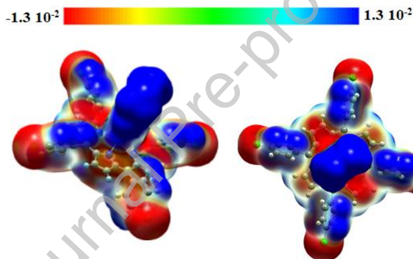
Figure 16. Molecular Electrostatic Potential (MEP) maps of the [Mg(TCIPP)(DMAP)] molecule.
