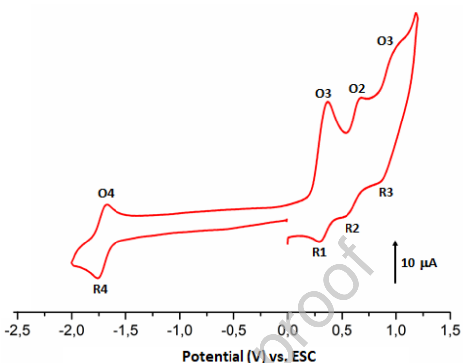
Figure 17. Cyclic voltammogram of (I). The solvent is CH 2 Cl 2 , and the concentration is ca. 10 -3 M in 0.2 M TBAP, 50 mV/s, vitreous carbon working electrode (Ø = 3 mm).
