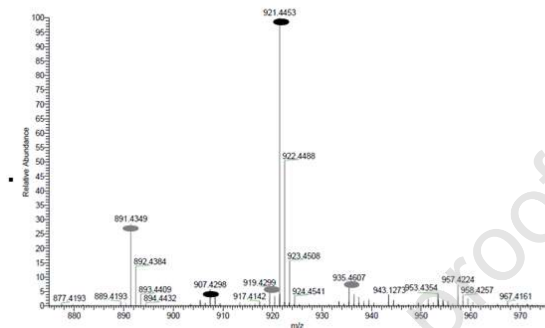
Fig. 4. ESI-MS mass spectrum (in the m/z 800 and 100 range) obtained for the MAE saponin extract from E. sepositus . MS signals marked by a black dot correspond to saponin congeners already identified in E. sepositus , while signals identified by gray dots could represent new saponins for this species.
