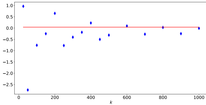
Figure 22: Determination of S_{1,1} for the spin-oscillator using Formula (44) with x = 0.01 and \mu = 1 , for different values of k . The red line corresponds to the theoretical result S_{1,1} = \frac{1}{8\pi} .
