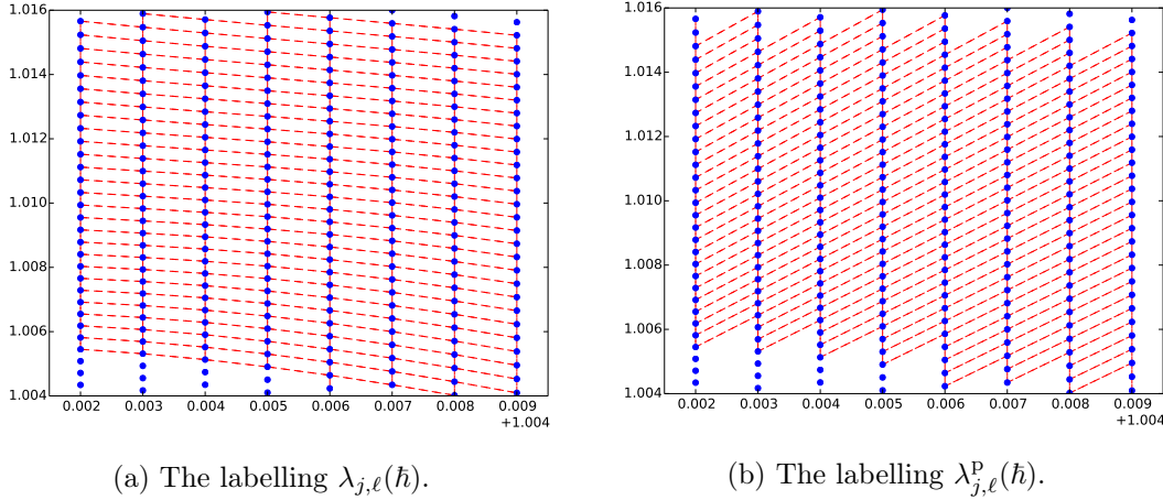
Figure 16: Two labellings of the joint spectrum near c = (1.01, 1.01) for the system (J, H+J) where (J, H) is the spin-oscillator system, for k = 1000 . Here s(0) = 1 and the approximate value of \sigma_1(0) given by Formula (27) evaluated at x = 0.01 with (j, \ell) = (0, 0) is \frac{E_{0,0} - E_{1,0}}{E_{0,1} - E_{0,0}} + \frac{1}{k(E_{0,1} - E_{0,0})} \approx 3.046 . The labellings are suggested by the red dashed lines.
