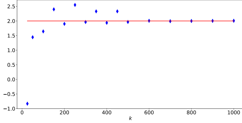
Figure 9: Determination of \partial_y f_r(0) for the spin-oscillator using Formula (20) with x = 0.01 , \mu = 2 and (j_1, \ell_1) = (0, 0) = (j_2, \ell_2) , for different values of k . The red line corresponds to the theoretical result \partial_y f_r(0) = 2 .
