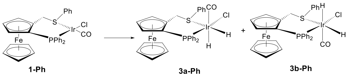
Scheme 3. H 2 addition to 1-Ph .
