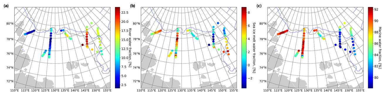
Figure 14. Fractions of river water (a), sea ice melt water (b), and marine water (c), calculated using \delta\text{-O}^{18} measurements and the Bauch and Cherniavskaya (2018) three-component model of freshwater balance. A thin black line shows the position of sea ice edge on 31 August 2018, when the northern stations of the meridional (5) transect along 126^\circ\text{E} were done in the MIZ, and the blue line shows the sea ice edge on 16 September 2020, when the ARKTIKA-2018 expedition was working in the MIZ of the East-Siberian Sea. Please note that the color bar scale is different for each water fraction.
