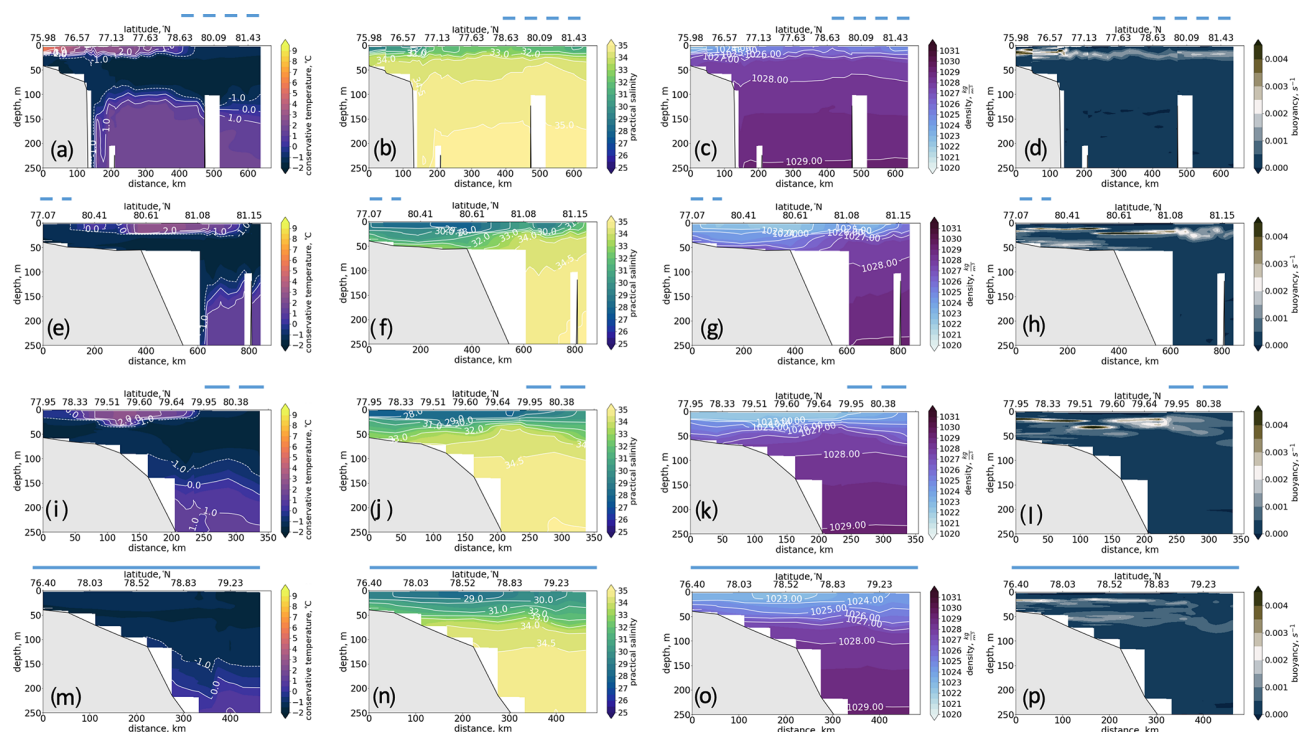
Figure 13. Conservative temperature (left, first column), practical salinity (second column), density (third column), and Brunt–Vaisala frequency (right, last column) in the upper 250 m along oceanographic transect 5 (a–d), transect 6 (e–h), transect 8 (i–l), and transect 7 (m–p). See Fig. 1 for the section positions. The 0 km point is always placed at the southern point of each transect. The dashed blue line indicates the MLD for transects 5, 6, and 8 (the rest is ice-free area); the full line indicated that transect 7 was done under the ice.
