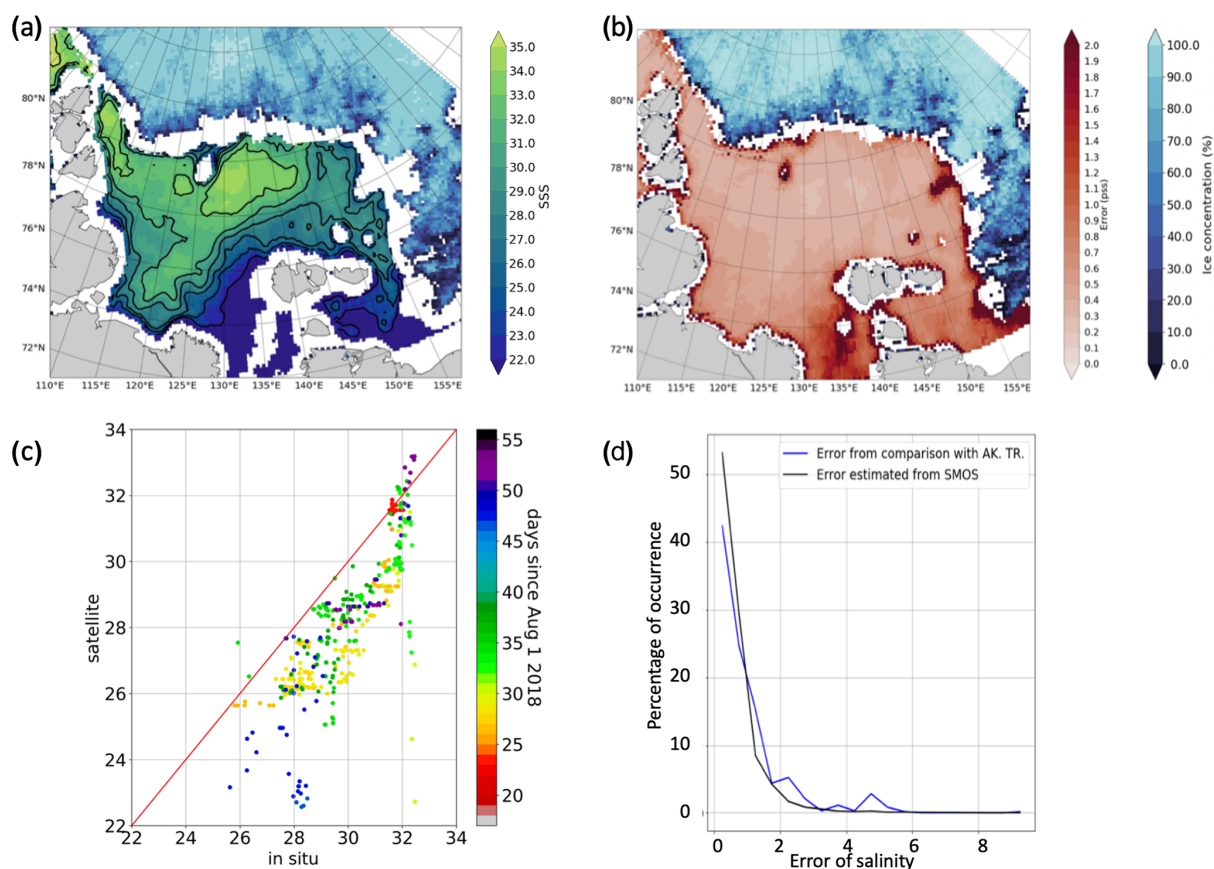
Figure 5. Sea surface salinity validation shown with an example of SMOS SSS “A” for 13 September 2018 (a) and associated uncertainties (b), a scatterplot of colocated SSS and in situ data in the upper 6.5 m (c), and statistical distribution of provided SMOS L2 uncertainties and measured absolute difference from comparison with in situ data (d). Sea ice concentration from AMSR2 is indicated with blue shading on the upper panels
