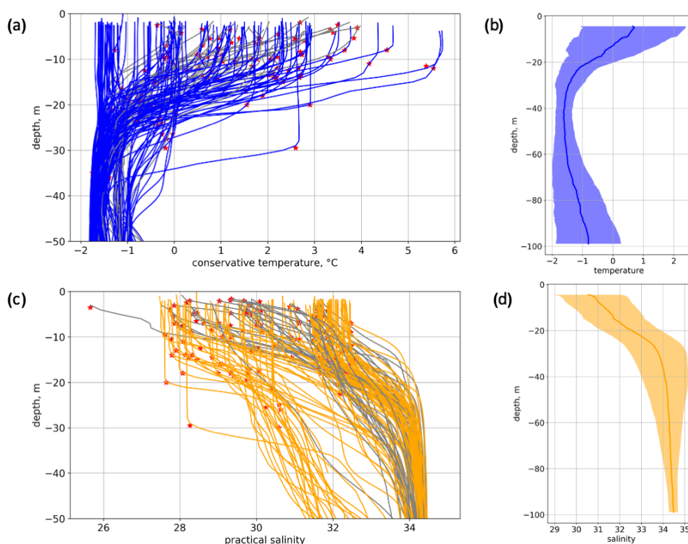
Figure 2. Vertical profiles of conservative temperature (a, b) and practical salinity (c, d) from CTD measurements in the upper ocean layer. Panels (a) and (c) show all vertical profiles in the upper 50 m, calculated using de Boyer Montégut et al. (2004) method (see details in the text); red stars indicate the mixed layer depth, colored profiles show the cases when the MLD is below 7 m depth, and gray profiles indicate when the MLD is above 7 m depth. Panels (b) and (d) show the median vertical profiles in the 5–100 m layer of temperature and salinity, respectively, where the shaded area shows the associated SD.
