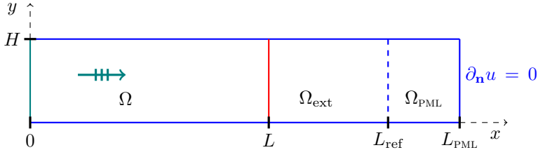
Figure 7: Illustration of the strategy to compute the reference solution. The mean flow derivative is assumed to be zero at x = L_{ref} . The ABC boundary is at x = L .
