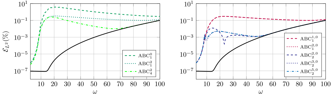
Figure 3: Relative L^2 -error for Taylor-based (left) and Padé-based (right) ABCs as a function of the input frequency \omega for \alpha = 0 and \varepsilon = 0 . Reference solution(—).
