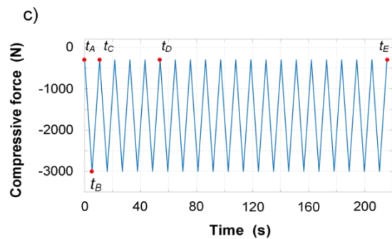
Figure 1. Experimental setup: a) picture of the device, b) a schematic view of the granular sample placed in the rectangular frame, and c) example of cyclic mechanical loading with five specific times used in the processing of the thermal data measured by the IR camera.
