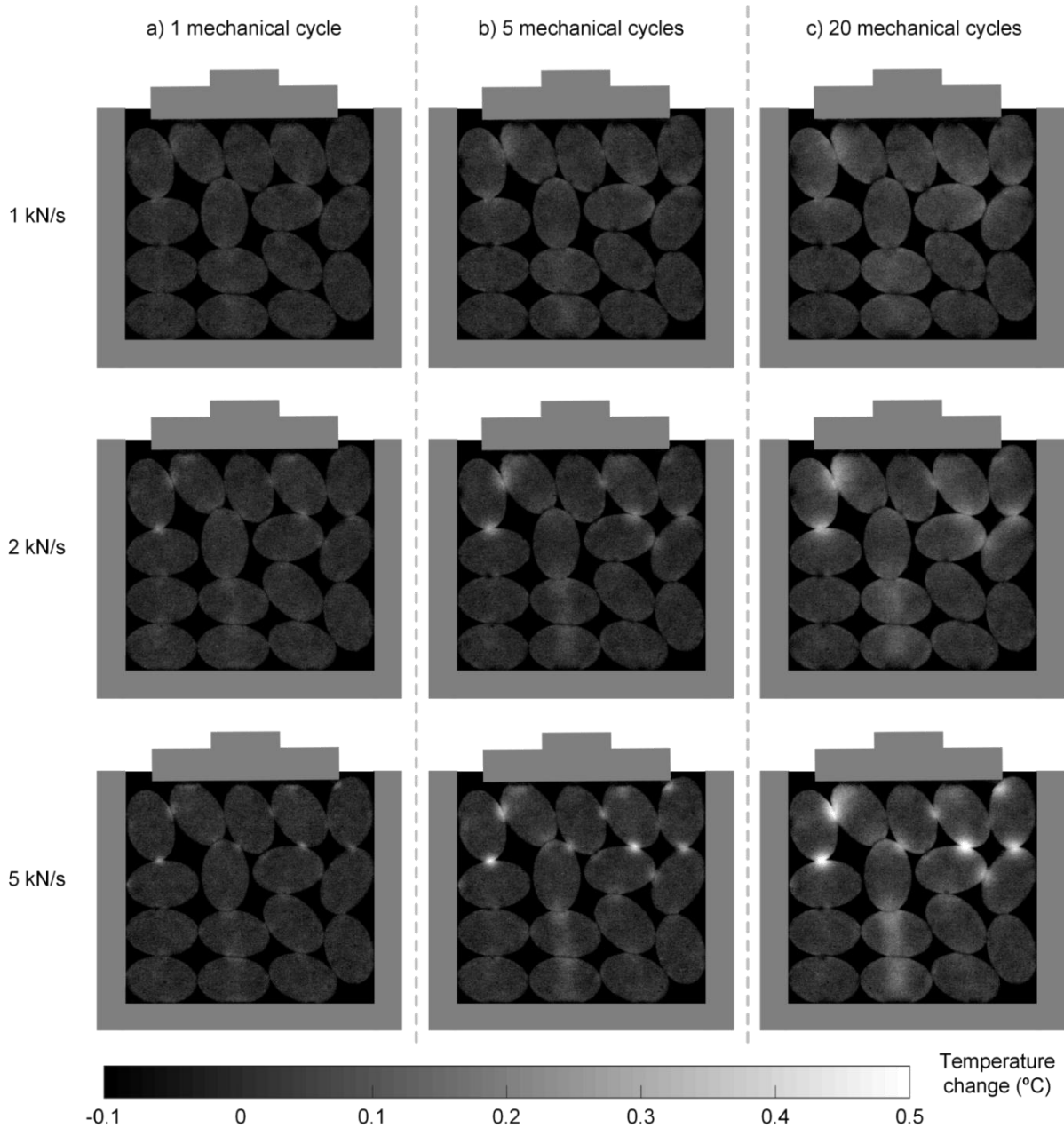
Figure 3. Fields of temperature change revealing mechanical dissipation: a) over one mechanical cycle from times t_A to t_C in Fig. 1-b, b) over five cycles from t_A to t_D , and c) over twenty cycles from t_A to t_E .
