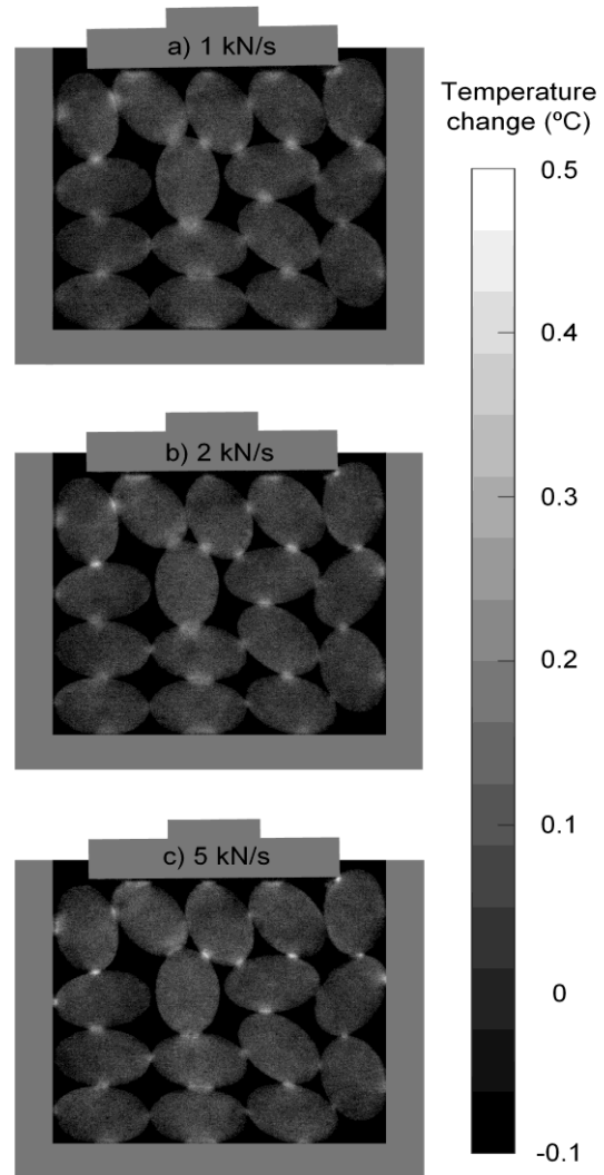
Figure 2. Fields of temperature change over half of the first mechanical cycle, revealing thermoelastic couplings: a) force rate of 1 kN/s, b) force rate of 2 kN/s, c) force rate of 5 kN/s.
