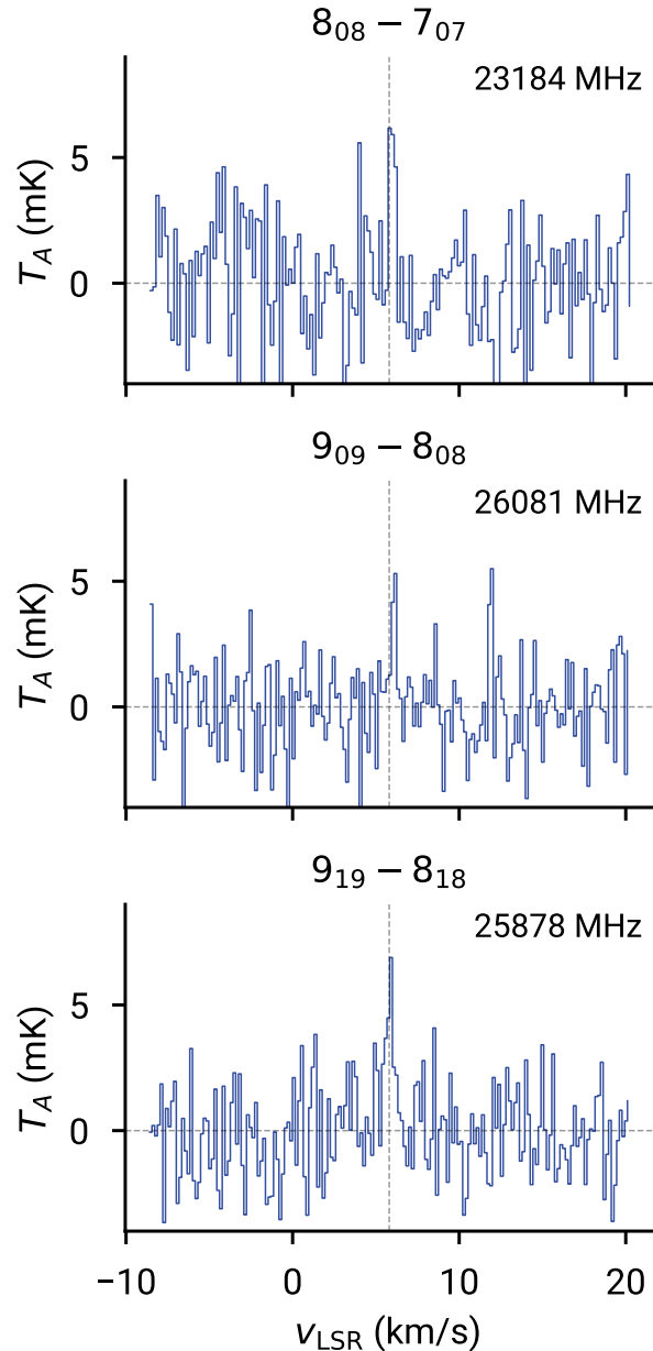
Figure 2. Observed spectral features in the GOTHAM spectrum (rebinned to 14 kHz resolution) at the center frequencies for three a -type transitions of trans -(E)-CVA. The dashed vertical line indicates the nominal source velocity at 5.8 km/s. Asymmetric top ( J_{K_a K_c} ) quantum number assignments are given at the top of each trace, along with their rest frequencies. The peak signal-to-noise ratio for each spectrum is on the order of \sim 3\sigma .
