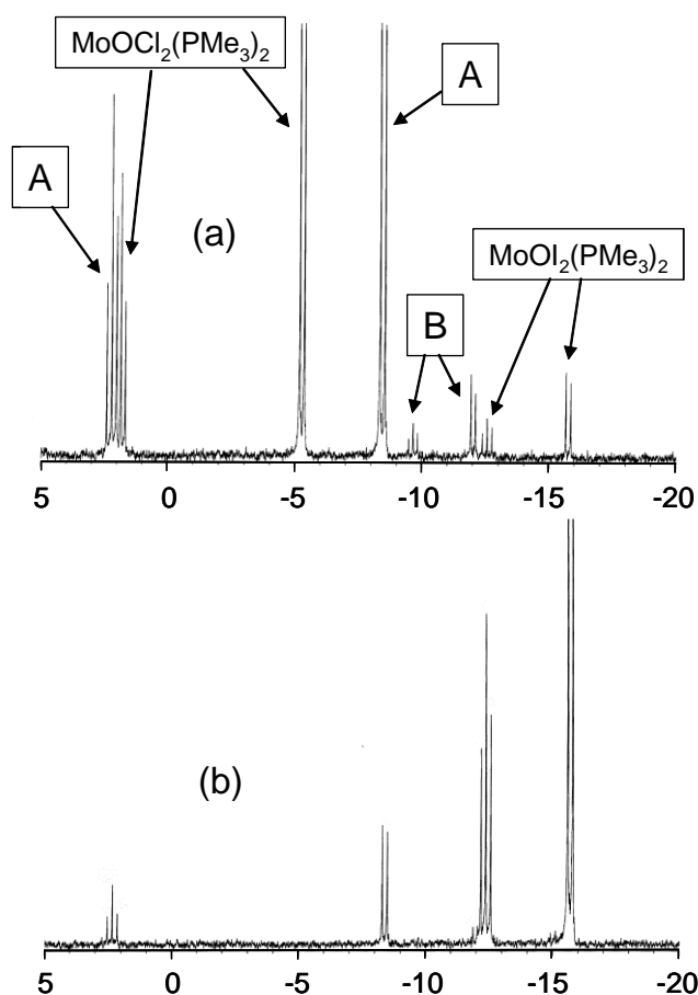
Figure 4. Room temperature ^{31}\text{P}\{^1\text{H}\} NMR spectra of \text{MoOCl}_2(\text{PMe}_3)_3 (50 mg, 0.12 mmol) and NaI in acetone- d_6 (0.6 mL). (a) After 5 h with 1 equiv NaI. (b) After 2.5 h from spectrum (a) with excess NaI.
