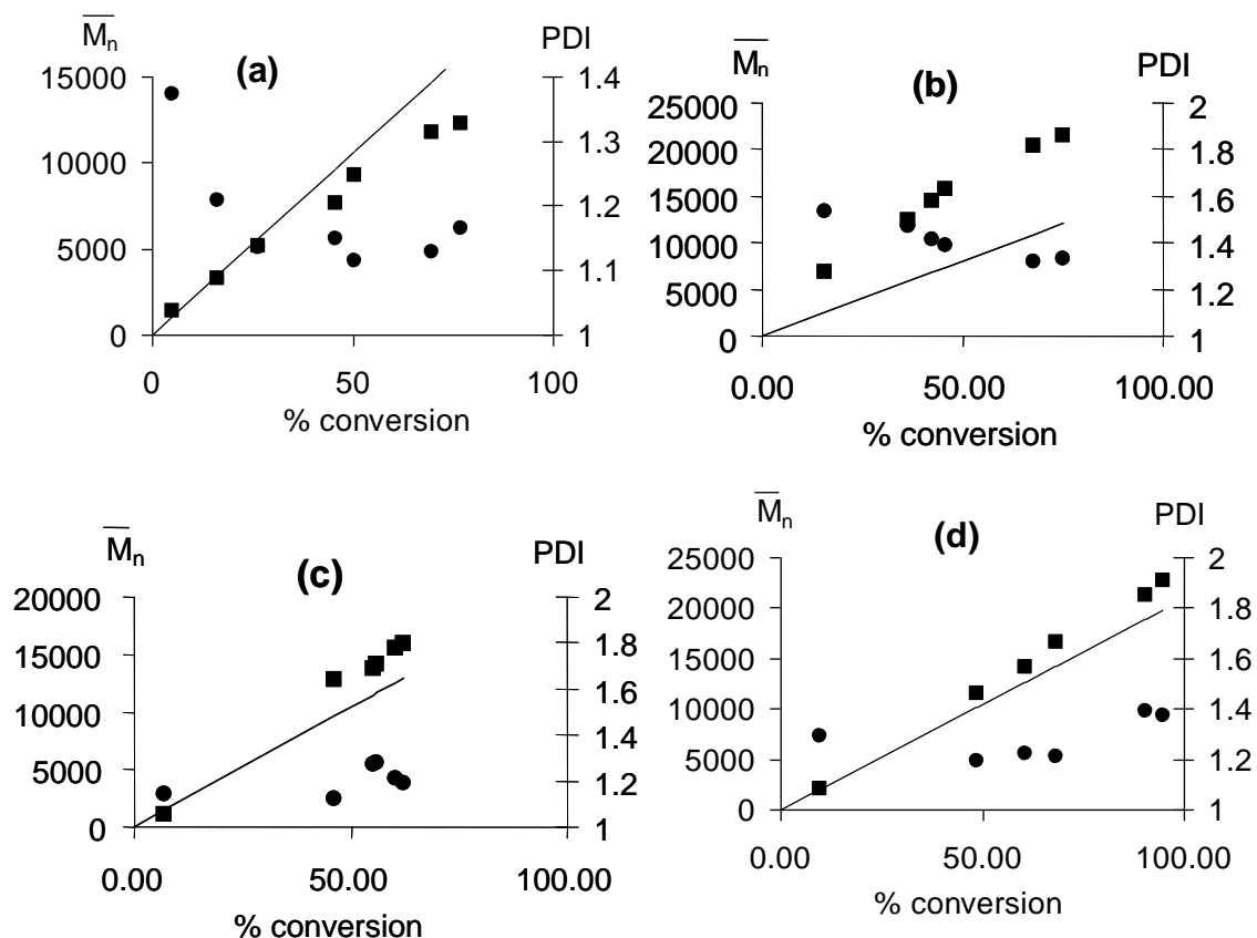
Figure 6. \bar{M}_n vs. conversion and PDI for the ATRP of styrene catalyzed by \text{MoOX}_2(\text{PMe}_3)_3 (X = Cl, I). The conditions are given in Table 3 (entries 1-4). Squares: experimental \bar{M}_n ; circles: PDI; straight line: theoretical \bar{M}_n . (a) X = Cl, no Al(O i Pr) 3 (entry 1); (b) X = Cl, with Al(O i Pr) 3 (entry 2); (c) X = I, no Al(O i Pr) 3 (entry 3); (d) X = I, with Al(O i Pr) 3 (entry 4).
