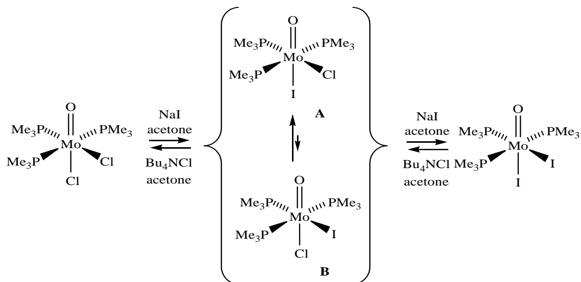
Scheme 5
