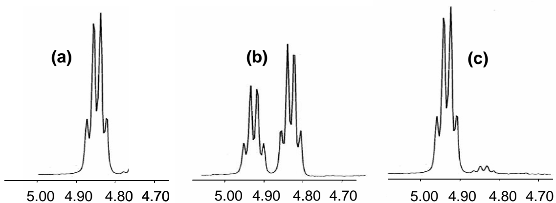
Figure 5. ^1\text{H} NMR monitoring of the halogen exchange between \text{MoOI}_2(\text{PMe}_3)_3 and BEB in toluene- d_8 at 90^\circ\text{C} ( [\text{Mo}] = [\text{BEB}] = \text{ca. } 0.1 \text{ mol l}^{-1} ). (a) t = 0 . (b) t = 20 \text{ min} . (c) t = 40 \text{ min} .
