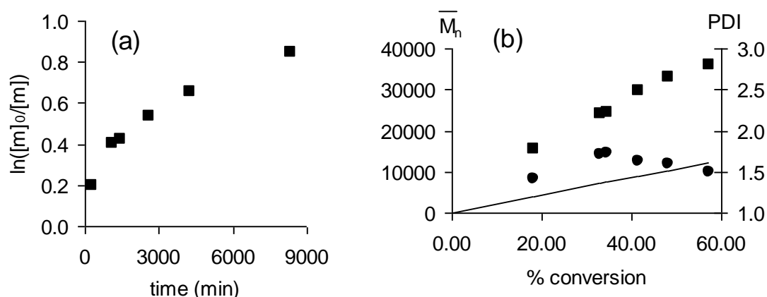
Figure 7. Polymerization of methyl acrylate catalyzed by \text{MoOCl}_2(\text{PMe}_3)_3 at 35°C. Conditions: Mo:I:Al:MA = 1:1:1:250 (MA = methyl acrylate; I (initiator) = ethyl 2-iodopropionate; Al = Al(O i Pr) 3 ). (a) Kinetics plot. (b) \bar{M}_n vs. conversion and PDI for the Squares: experimental \bar{M}_n ; circles: PDI; straight line: theoretical \bar{M}_n .
