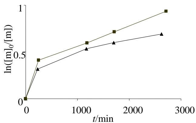
Figure 8. Polymerization of styrene in toluene (30% v/v) in the presence of the AIBN initiator (styrene/AIBN = 250) at 80°C. Squares: without Mo complex; triangles: with \text{MoOI}_2(\text{PMe}_3)_3 (AIBN/Mo = 1:1).
