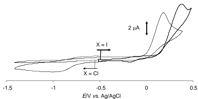
Figure 3. Cyclic voltammogram of compounds \text{MoOX}_2(\text{PMe}_3)_3 in THF. Thinner curve: \text{X} = \text{Cl} ; thicker curve: \text{X} = \text{I} . C_{\text{Mo}} = 4 \cdot 10^{-3} \text{ M} . Scan rate = 100 \text{ mV s}^{-1} .
