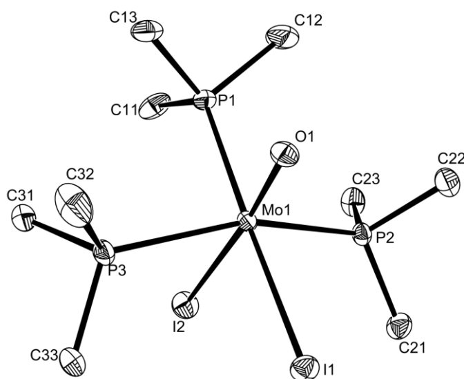
Figure 2. An ORTEP view of complex \text{MoOI}_2(\text{PMe}_3)_3 . The ellipsoids are drawn at the 50% probability level.
