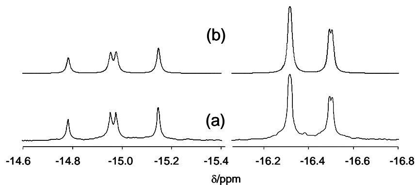
Figure 1. Experimental (a) and simulated (b) ^{31}\text{P} -NMR spectrum of compound \text{MoOI}_2(\text{PMe}_3)_3 in \text{C}_6\text{D}_6 .
