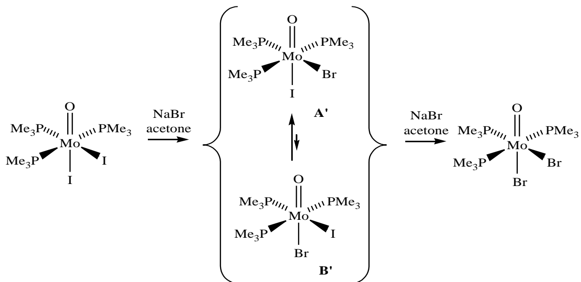
Scheme 6
