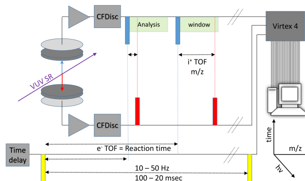
FIG. 7. Schematics of the detection setup and timing. Yellow signals represent the periodic excimer laser trigger, while blue and red bars represent the continuous arrival of electron and ion signals resulting from synchrotron photoionization. Ions within the analysis window are considered correlated to the electron that triggers the window.
