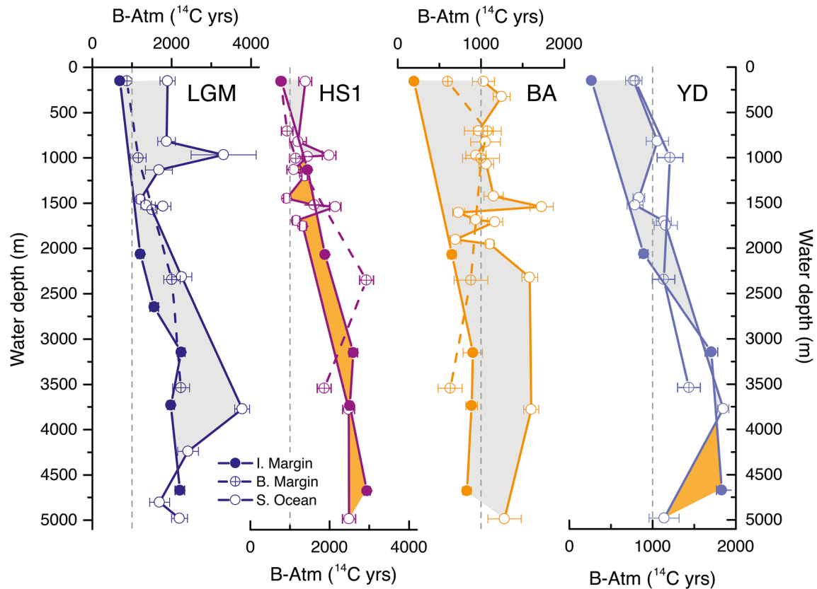
Figure 6. Depth profiles of ventilation age (B-Atm) for time-slices across the last deglaciation, from the Iberian Margin (filled symbols), Brazil Margin (crossed symbols), and Southern Ocean (open symbols; Zhao et al., 2018). The offset between the Iberian Margin (North Atlantic) and Southern Ocean is shaded (gray/orange indicates higher/lower B-Atm in the Southern Ocean), in order to illustrate periods where the radiocarbon ventilation gradient across the Atlantic collapsed or reversed, suggesting diminished supply of NADW to the Atlantic interior (i.e., during HS1, and to a lesser extent the YD). Despite overall reduced radiocarbon ventilation throughout the deep Atlantic, the ventilation gradient across the Atlantic at the LGM suggests active NADW export. HS1, Heinrich Stadial 1; LGM, Last Glacial Maximum; NADW, North Atlantic Deep Water; YD, Younger Dryas.
