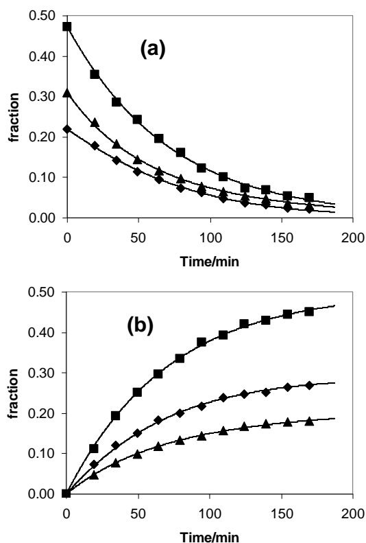
Figure 7. Evolution of the concentrations of (a) nonclassical and (b) classical complexes during the isomerization process following the reaction of Cp*Fe(dppe)H with CF 3 COOD at
