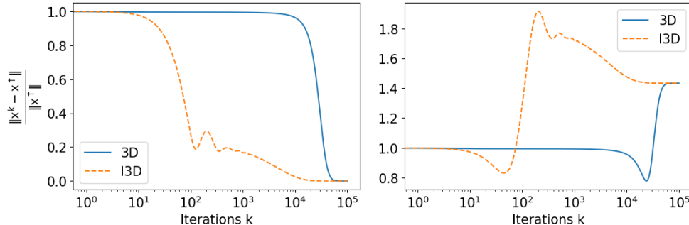
Figure 2: Illustration of two iterative regularization methods (Dual Diagonal Descent (3D) [43] and its Inertial variant (I3D) proposed in this work) on a simple problem. Left: given the true data \bar{y} , the iterates converge to the ideal solution x^\dagger . Right: given noisy data \hat{y} , the iterates x_k(\hat{y}) =: \hat{x}_k approach x^\dagger before tending away from it. Regularization holds by early stopping the algorithms at a suitably chosen iterate k^* . In this example, k^* \simeq 2 \times 10^4 (resp. 50) minimizes \|\hat{x}_k - x^\dagger\| for (3D) (resp. (I3D) ).
