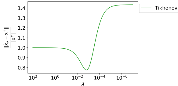
Figure 1: Tikhonov regularization path on a simple problem. After computing the solution \hat{x}_\lambda := x_\lambda(\hat{y}) of the problem (\mathbf{P}_\lambda(\hat{y})) for several values of \lambda , the best parameter \lambda is selected. In this example, \lambda \simeq 10^{-3} minimizes \|\hat{x}_\lambda - x^\dagger\| .
