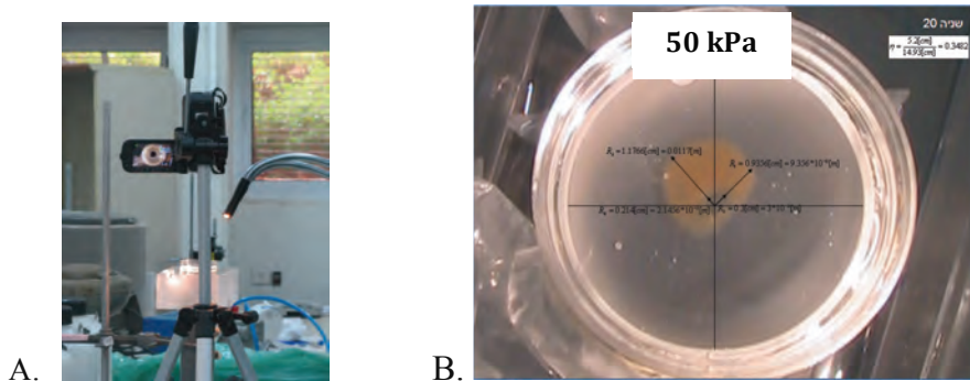
Figure 5 - Evaluating streaming and microstreaming in the plate above the cells. A) The apparatus that was used to estimate the generated streaming field in the US system; B) An example for the coffee stain dimensions.
