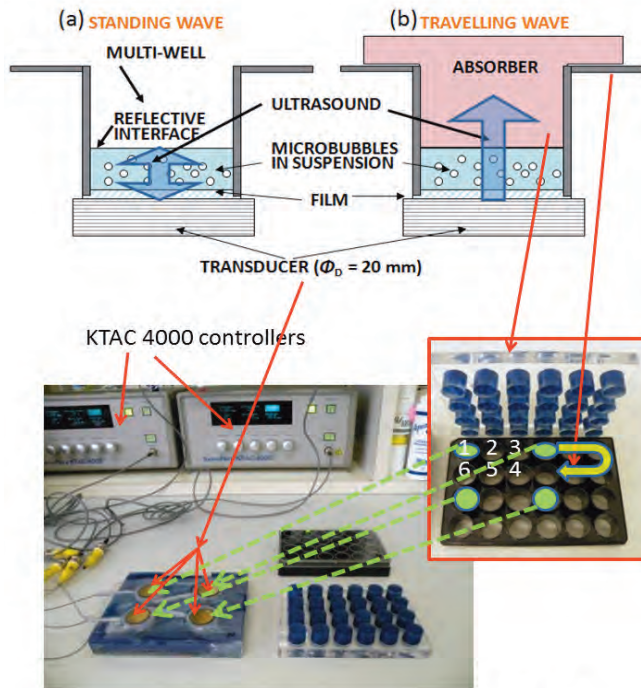
(c) Transducer array mat and absorber array to fit 24 well plate. (inset – above right) Green spots indicate where transducers map over 4 individual wells simultaneously.
