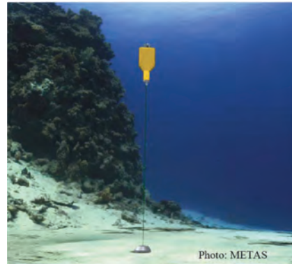
Figure 12 - COMPEC Acoustic buoy (METAS).
