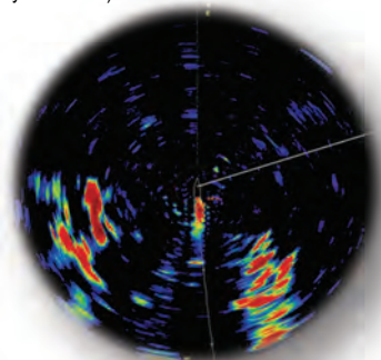
Figure 4 - A Simrad SP90 sonar showing shoal fish on both side of the ship.
