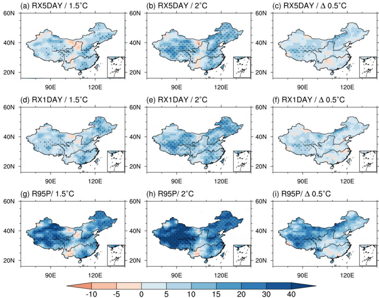
Fig. 10. Percentage changes of the three extreme precipitation indices projected by PI-based weighting scheme for the 1.5°C (first column), 2°C (second column) global warming under RCP 8.5 scenario compared to the period 1985-2005 and the additional 0.5 °C warming (third column). Areas with significant changes above 95% confidence level are marked with black dots (unit: %).
