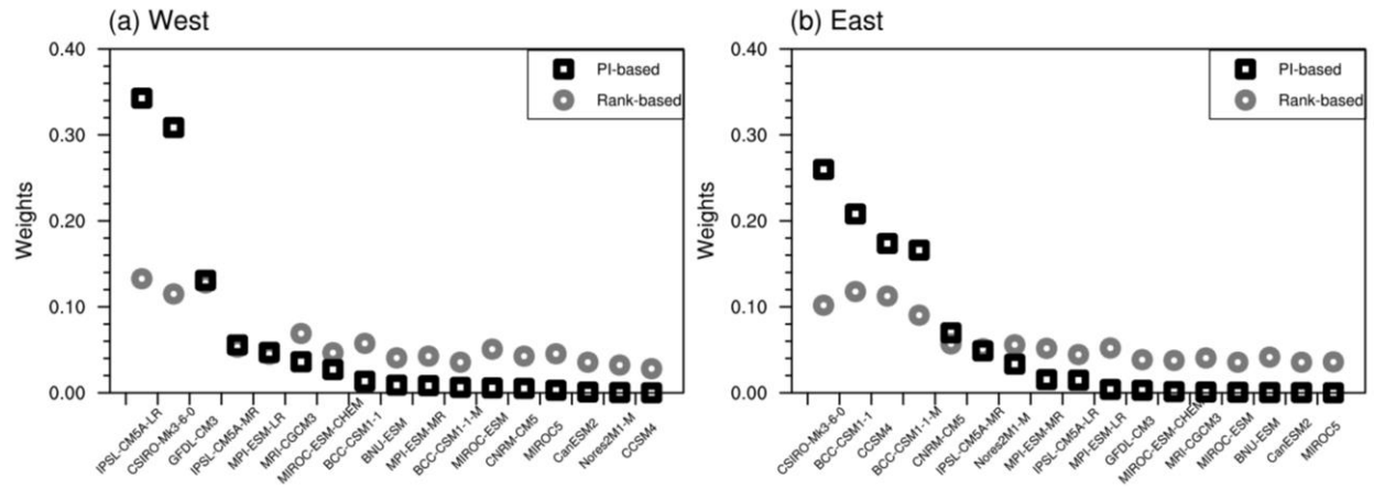
Fig. 3. The models' weights obtained by PI-based weighting scheme (black squares) and Rank-based weighting scheme (gray circles) over (a) western and (b) eastern China.
