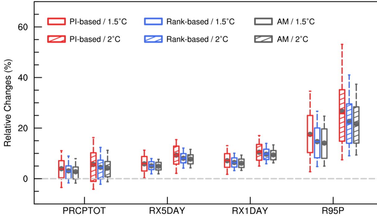
Fig. 7. Boxplot for relative changes of total precipitation and extreme indices (compared to the period of 1985-2005) from PI-based, Rank-based weighting schemes and AM over China under 1.5°C and 2°C global warming (unit: %).
