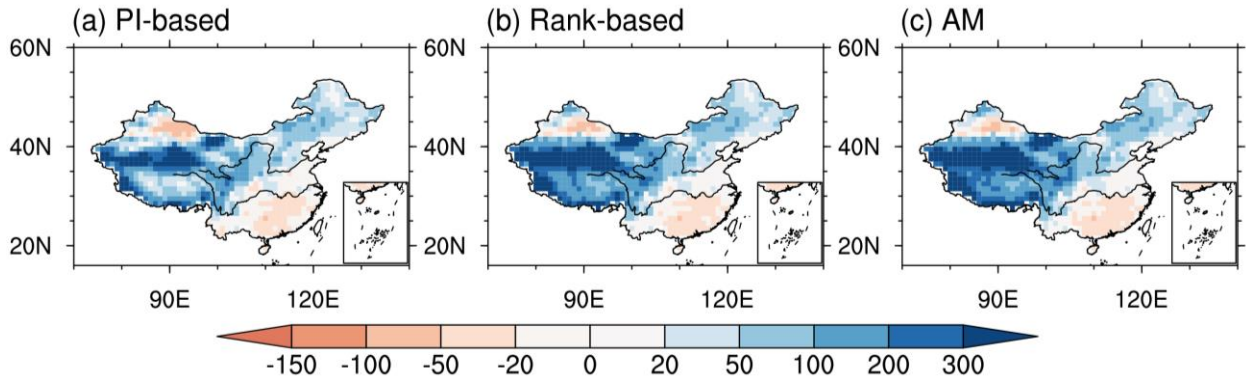
Fig. 5. Spatial distribution of relative bias for R95P from (a) PI-based (b) Rank-based and (c) AM schemes against observations during the period 1986-2005 (unit: %). Warm and cool colors indicate dry and wet bias respectively.
