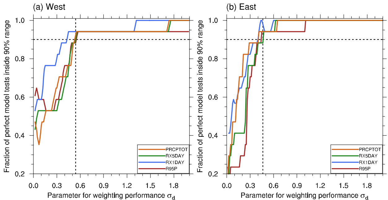
Fig. 2. The fraction of cases for four indices when the actual outcomes of the perfect model tests are in the 5 th -95 th range weighted by all other models. For all indices, the minimum value of \sigma_d for the fraction expected to exceed 90%.
