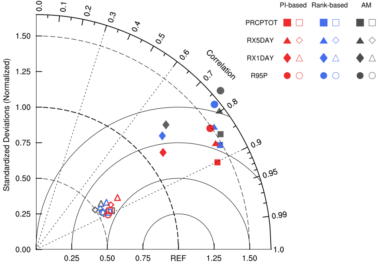
Fig. 6. Taylor diagram showing the four precipitation indices under the three weighting schemes during the period 1986-2005. The solid and hollow markers represent western and eastern China respectively.
