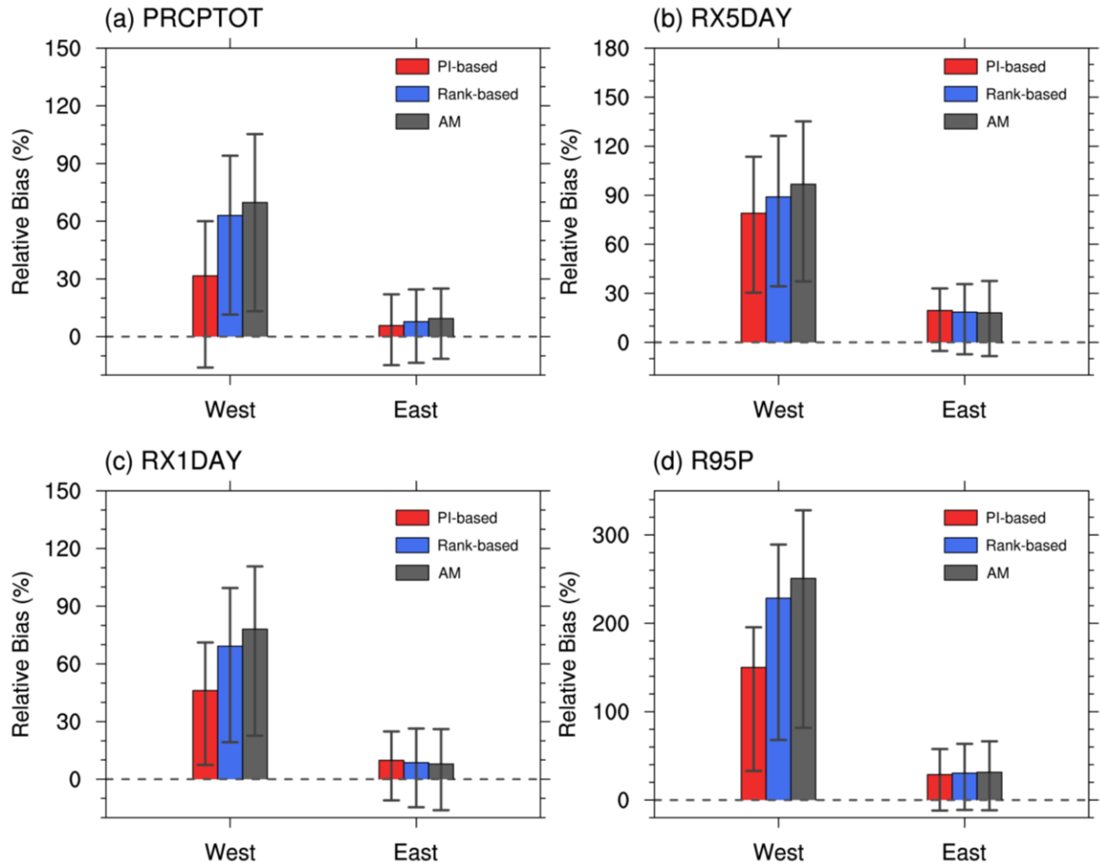
Fig. 4. The regional relative bias simulated by PI-based, Rank-based and AM schemes against observations for four precipitation indices during the period of 1986-2005. Color bars are the mean biases and whiskers represent the first and third quartiles (unit: %).
