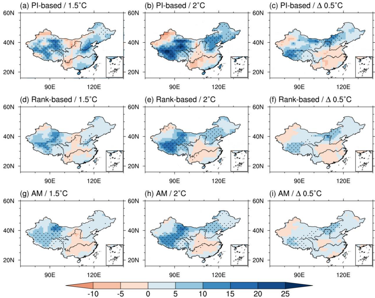
Fig. 9. Percent changes of PRCPTOT for the 1.5°C (first column), 2°C (second column) global warming under RCP 8.5 scenario compared to the period 1985–2005 and the additional 0.5 °C warming (third column) from simulations of PI-based (top), Rank-based (middle) weighting schemes and AM (bottom). Areas with significant changes above 95% confidence level are marked with black dots (unit: %).
