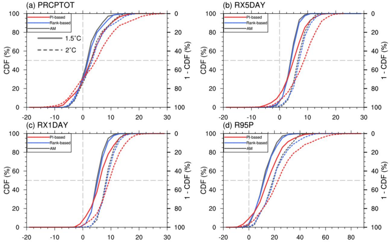
Fig. 8. The spatial fraction CDFs of changes weighted by PI-based, Rank-based and AM under 1.5°C and 2°C global warming for the indices over China. The abscissa displays the changes of precipitation indices while the left ordinate shows the CDF values, the complementary values (1-CDF) shown on the right side. The changes are expressed by percentages (%) compared to the period of 1985-2005.
