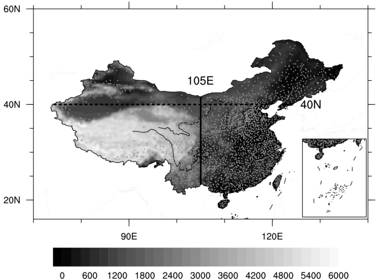
Fig. 1. Topography and location of surface weather stations in China.
