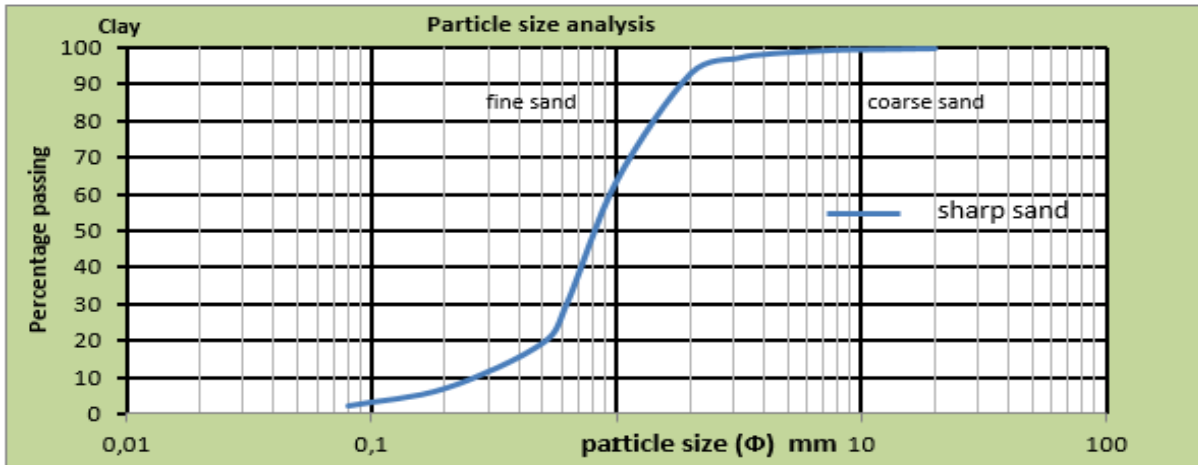
4 Figure 1. Sanaga River sand granulometric analysis curve.
