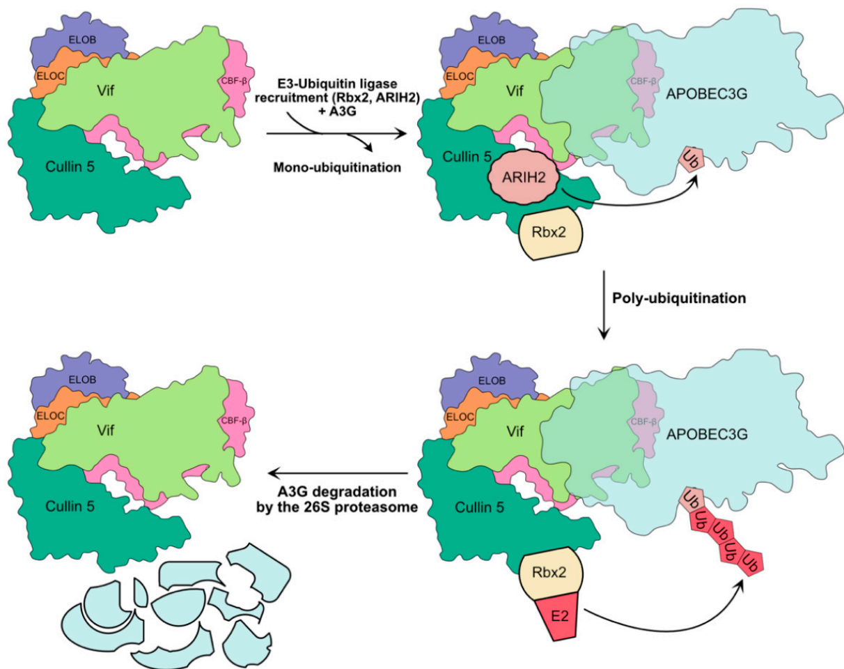
Figure 3. Hijacking of ubiquitin–proteasome pathway by Vif. HIV-1 first recruits the core components of the E3-ubiquitin ligase complex, namely Elongin B (ELOB) and ELOC, CBF- \beta , and Cullin 5. This complex is represented in accordance with its known 3D structure (PDB: 4N9F). The recruitment of A3G and catalytic subunits Rbx2 and ARIH2 leads to ARIH-2 mediated mono-ubiquitination of A3G. Subsequent recruitment of an E2 ubiquitin-conjugating enzyme by RBX2 leads to the poly-ubiquitination of A3G and its degradation by the 26S proteasome.
