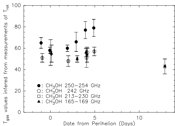
Fig. 10. Daily gas temperatures T_{\text{gas}} derived from the methanol rotational lines around 167, 213–230, 242, and 252 GHz as presented in the first part of Table 3. Variations cannot be related to the rotation of the nucleus (when folded on a single 9 h period). Most of the dispersion is due to the different series of methanol lines used: the 252 GHz ones sample a smaller region than the others and keep memory of T_{\text{gas}} at larger cometocentric distances than those at 242 GHz.
