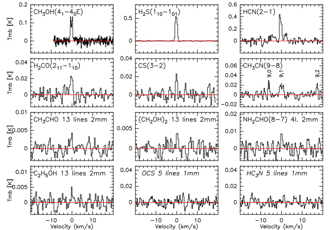
Fig. 3. Molecular lines observed in comet 46P/Wirtanen between 11.9 and 18.1 Dec 2018 in the 2 mm band, except for \text{HC}_3\text{N} and \text{OCS} , for which we show the weighted average of five lines expected in the 1 mm band. For some complex organics, we averaged several lines between 147 and 170 GHz (2 mm wavelength). The vertical scale is the main beam brightness temperature and the horizontal scale is the Doppler velocity in the comet rest frame.
