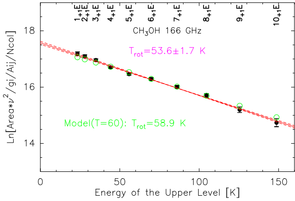
Fig. 6. Rotational diagram of the 13–17 Dec average of the methanol lines around 166 GHz in comet 46P/Wirtanen. The neperian logarithm of a quantity proportional to the line intensity is plotted against the energy of the upper level of each transition. Fit is shown by solid red line and errors are displayed by red dashed lines. The black dots are the measurements and green circles the predicted values for a model with a gas temperature of 60 K.
