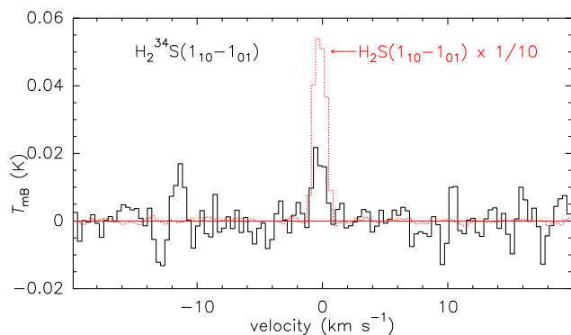
Fig. 13. \text{H}_2^{34}\text{S}(1_{10}-1_{01}) line at 167910.516 MHz together with the main isotopologue \text{H}_2^{32}\text{S} line divided by 10 and observed in the same FTS spectrum between 13.0 and 17.0 Dec 2018. The vertical scale is the main beam brightness temperature, and the horizontal scale is the Doppler velocity in the comet rest frame. The feature at -11 \text{ km s}^{-1} does not correspond to any known molecular line and could be spurious.
