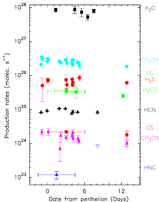
Fig. 12. Evolution of production rates in comet 46P/Wirtanen between 12 and 25 December 2019 (perihelion was on 12.9 Dec.) for the nine main molecules. Downward-pointing empty triangles are 3\text{-}\sigma upper limits. Coloured symbols are in the vertical order of the corresponding molecules' names on the right. Water production rates have been computed from data in Lis et al. (2019).
