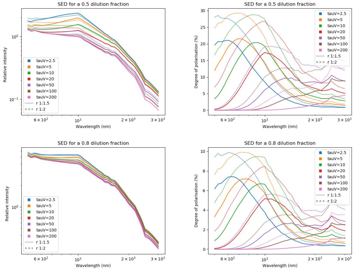
Fig. 12. Spectra of relative intensity ( first column ) and degree of polarisation ( second column ) for an AGN with dilution fractions of 50% ( first row ) and 80% ( second row ) from MontAGN simulations. Intensity is normalised to the maximum of the dichroic flux as detailed in text.
