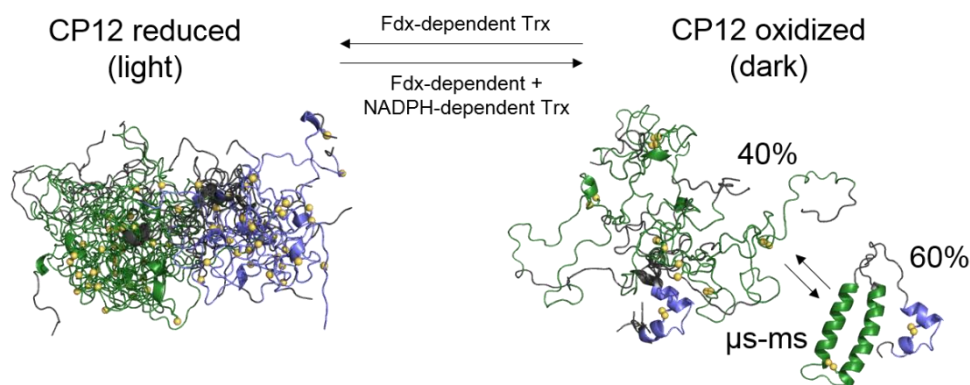
Figure 1: Model of the redox-transition of CP12. The structural models are derived from Launay et al [30,31]. The complex Trx network is derived from Cejudo et al [15]. The sulphur atoms of the two pairs of cysteine residues are in yellow. Trx and Fdx stand for thioredoxins and ferredoxin respectively.
