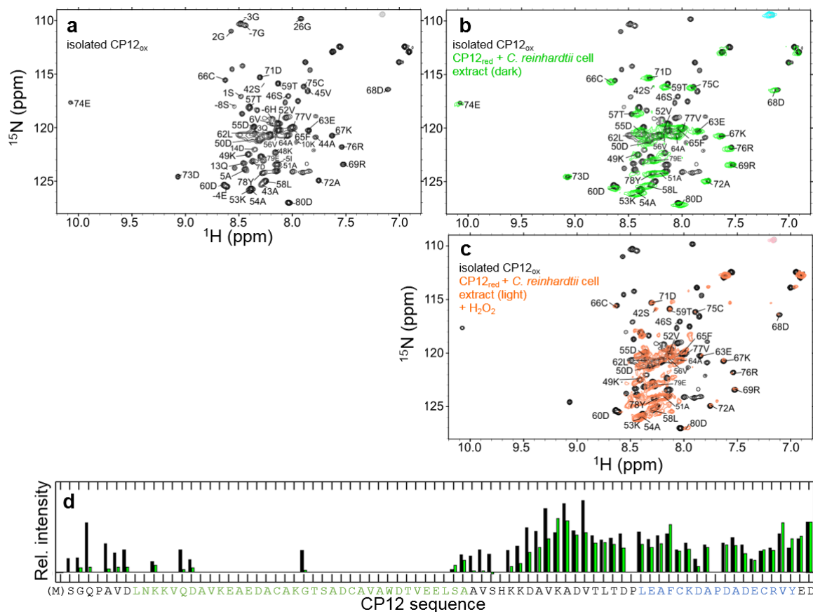
Figure 5: CP12 ox in isolation and in presence of C. reinhardtii cell extract. (a) 1 H- 15 N HSQC spectrum of isolated CP12 ox . (b) overlay of the 1 H- 15 N HSQC spectra of isolated CP12 ox (black) and that of CP12 in presence of C. reinhardtii cell extract (green, molecular crowding corresponding to 19 mg/mL of proteins). The data is recorded in the presence of 20 mM DTT ox , and 0.1 mM DCMU. The assignments of the resonances that are observed in the presence of cell extract are indicated. (c) 1 H- 15 N HSQC of CP12 in presence of C. reinhardtii cell extract collected in the light (molecular crowding corresponding to 15 mg/mL of proteins) and 20 mM H 2 O 2 as a strong oxidizing agent. (d) Signal intensities for all
