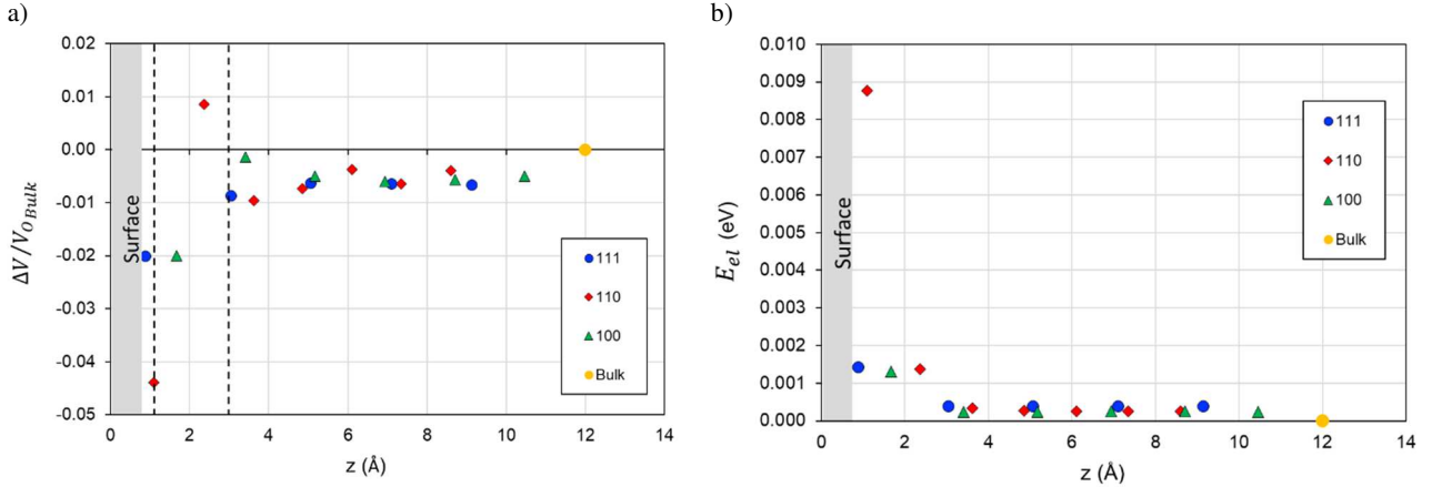
Figure 8: a) Local volume dilatation of O sites depending on their z-distance to {100}, {110} and {111} surfaces and b) associated internal elastic energies, compared to the unstressed bulk reference (O site in relaxed conventional cell).
