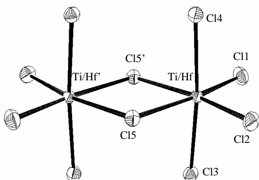
Figure 2. ORTEP view of the mixed-metal [\text{Ti}_{1.37}\text{Hf}_{0.63}\text{Cl}_{10}]^{2-} anion..
