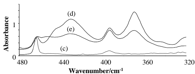
Figure 1. Far IR spectra of PPN salts in \text{CH}_2\text{Cl}_2 . All spectra are taken at the same \text{PPN}^+ cation concentration ( 10^{-2} M). (a) [\text{PPN}]_2[\text{Ti}_2\text{Cl}_{10}] ; (b) [\text{PPN}]_2[\text{Hf}_2\text{Cl}_{10}] ; (c) [\text{PPN}]\text{Cl} ; (d) electronic average of [\text{PPN}]_2[\text{Ti}_2\text{Cl}_{10}] + [\text{PPN}]_2[\text{Hf}_2\text{Cl}_{10}] ; (e) 1:1 mixture of [\text{PPN}]_2[\text{Ti}_2\text{Cl}_{10}] and [\text{PPN}]_2[\text{Hf}_2\text{Cl}_{10}] .
