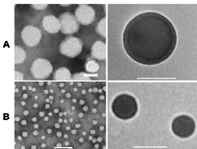
Figure 3: Transmission electronic microscopy of R-C nanoparticles (raw A) and R-CP nanoparticles (raw B). For observation at low magnification the nanoparticles were stained with phosphotungstic acid for 1 min. Nanoparticles observed at high magnification were stained with phosphotungstic acid for 30 s. Scale bar: 100 nm
