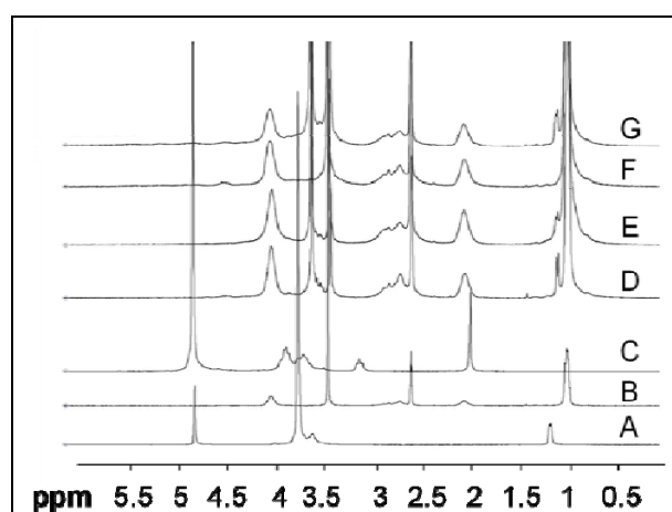
Figure 4: ^1\text{H} NMR spectra of pluronic F68 (A); of PIBCA (B); of chitosan (C); A-P nanoparticles (D); R-P nanoparticles (E); R-C nanoparticles (F); R-CP nanoparticles (G).
