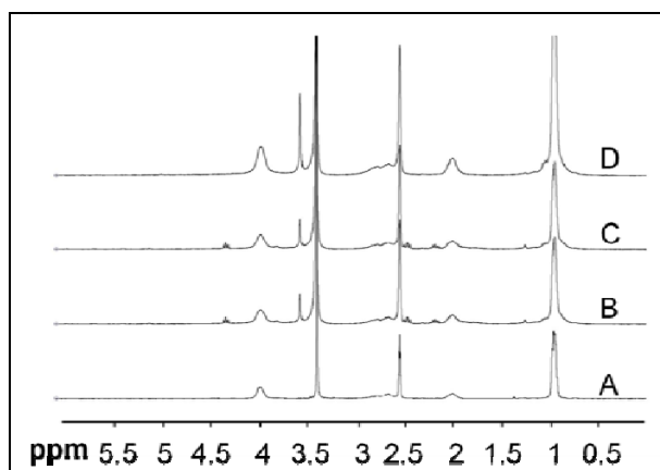
Figure 6: ^1\text{H} NMR spectra of PIBCA (A) and after acid hydrolysis of R-CP nanoparticles (B); R-C nanoparticles (C) and R-P nanoparticles (D).
