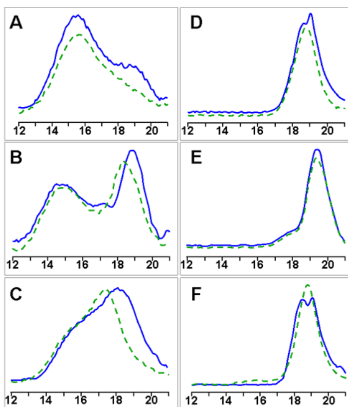
Figure 5: Chromatograms given by SEC profile given by the analysis of the THF soluble polymer composing nanoparticles (solid line) and of polymer recovered after acid hydrolysis of the nanoparticles (dotted line). A: R-CP nanoparticles, B: R-C nanoparticles, C: R-P nanoparticles, D: A-CP nanoparticles, E: A-C nanoparticles, F: A-P nanoparticles.
