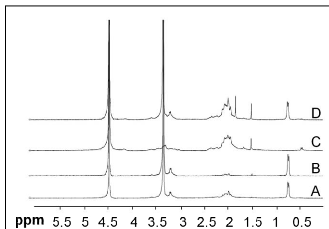
Figure 7: 1 H NMR after basic hydrolysis with NaOH of R-P nanoparticles (A); of A-P nanoparticles (B) of R-C nanoparticles (C) and of R-CP nanoparticles (D).
