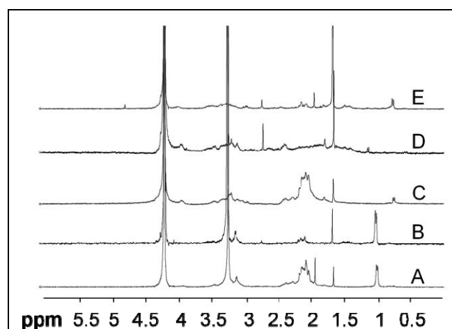
Figure 8: 1 H NMR spectra after hydrolysis with NaOH of R-CP nanoparticles (A), hydrolysis with NaOH and SPE filtration of R-PC nanoparticles (B), hydrolysis with NaOH of R-C nanoparticles (C), hydrolysis with NaOH and SPE filtration of R-C nanoparticles (D), after hydrolysis with NaH and SPE filtration of R-C nanoparticles (E).
