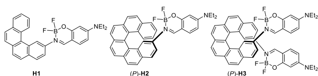
Figure 2. Chemical structures of new helicene-boranils presented in this work.
