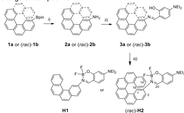
Scheme 1. Synthesis of helicene-boranils H1-H2 from helicene-boronates 1a-1b . i ) Na 3 , CuSO 4 ·5H 2 O, MeOH, reflux, 19 hrs, then H 2 , 10% Pd/C, EtOAc rt, 24 hrs, 2a : 65%, 2b : 75%; ii ) 4-(diethylamino)salicylaldehyde, MeOH, reflux, 3a : 18 hrs, 91%, 3b : 31 hrs, 93%; iii ) BF 3 ·OEt 2 , DIEA, 1,2-DCE, 85°C, H1 : 42 hrs, 75%, ( rac )- H2 : 24 hrs, 75%.
