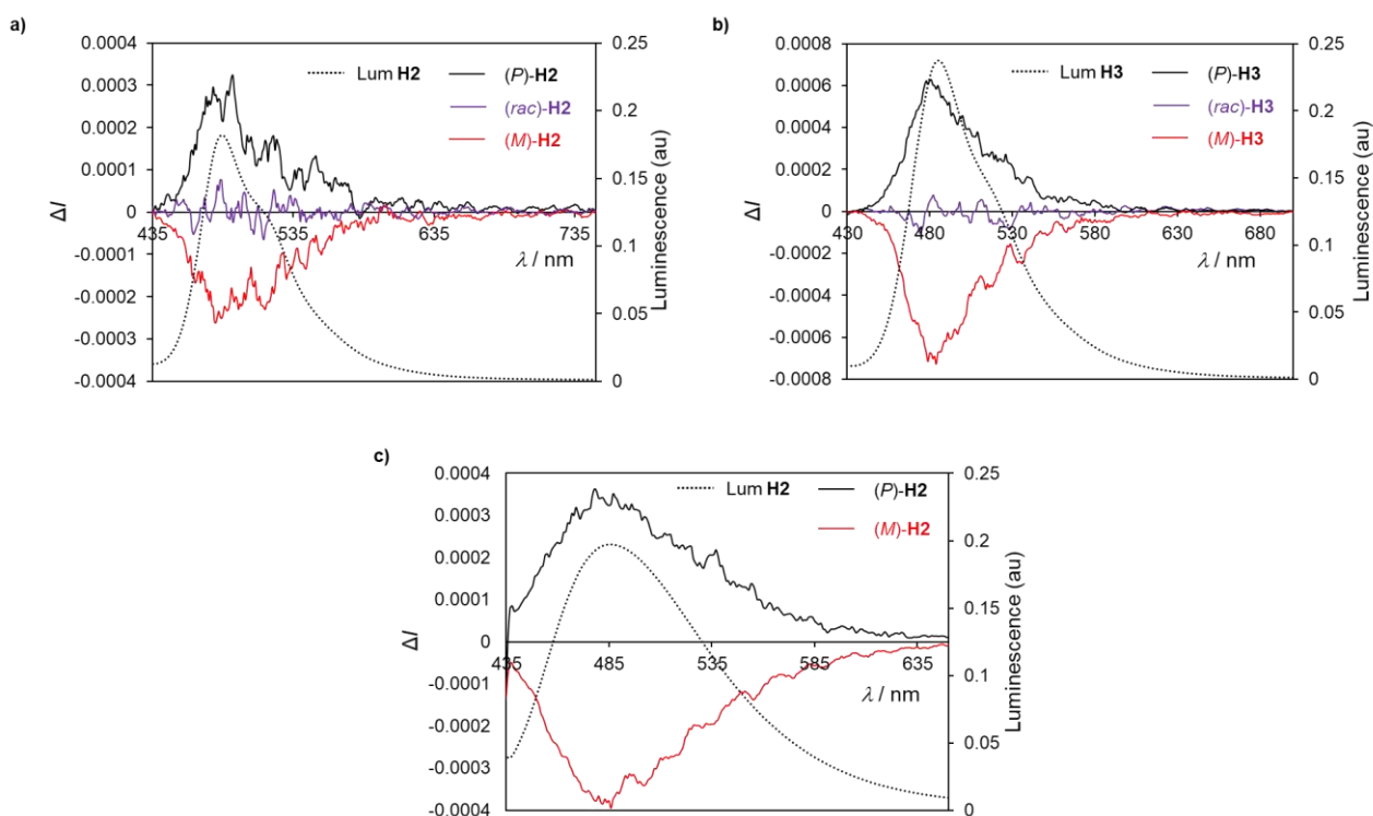
Figure 5. Experimental emission and CPL spectra of ( P ) and ( M ) enantiomers of a) H2 and b) H3 in \text{CH}_2\text{Cl}_2 at C \sim 10^{-5} M and rt and c) H2 in PMMA. Excitation wavelengths are 390 and 385 nm, for H2 and H3 , respectively.
