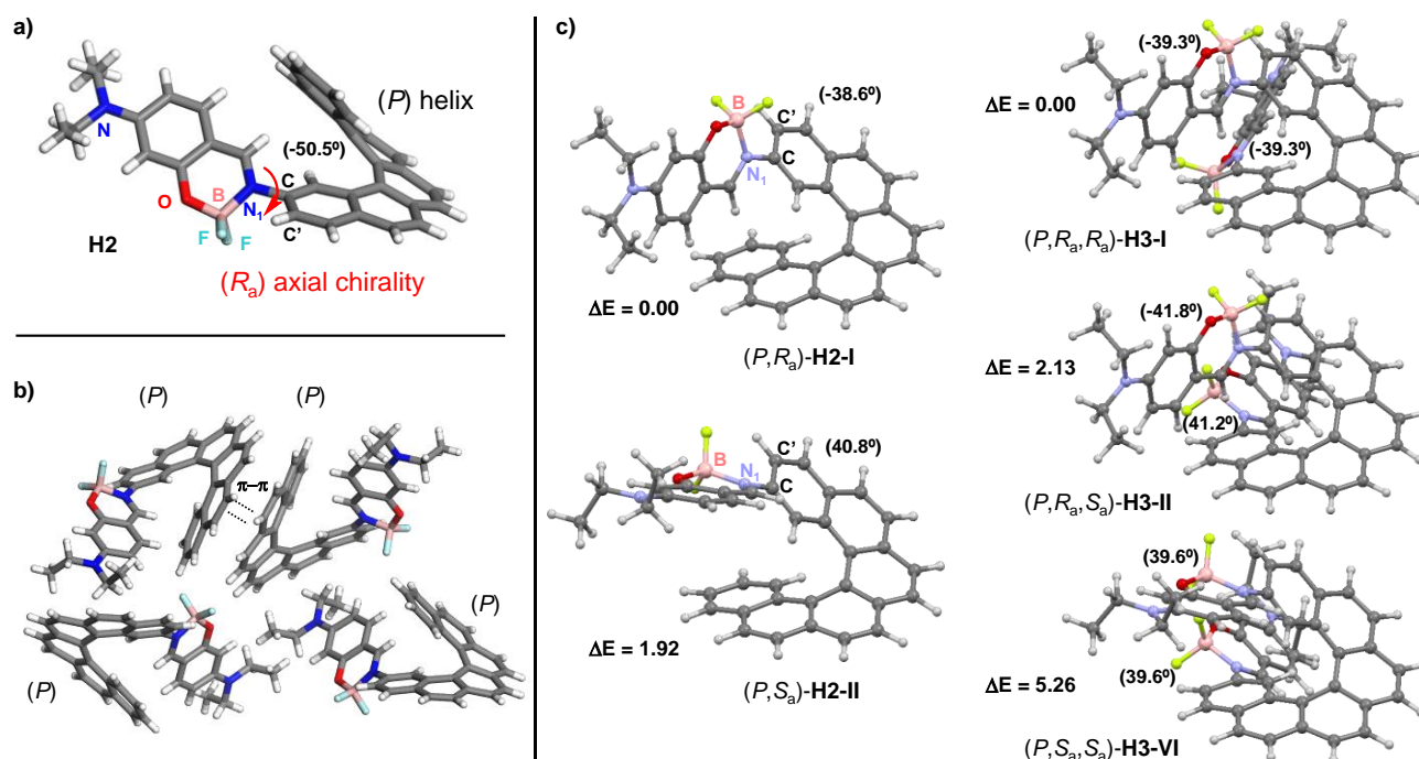
Figure 3. a) X-ray diffraction structure of (P) -(+)- H2 with (R_a) axial chirality highlighted along with b) its supramolecular arrangement in the crystal. c) Selected optimized (BP/SV(P) with the continuum solvent model for \text{CH}_2\text{Cl}_2 ) structures of H2 (left) and H3 (right). Compare with Table 2 and see Supplementary Information for a full set of data. Values listed are the corresponding relative energies \Delta E (in kcal/mol) calculated with BP-D3/TZVP and the B-N 1 -C-C' dihedral angles (provided in parentheses).
