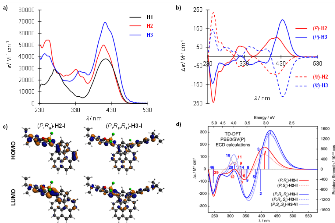
Figure 4. Experimental a) UV-vis of H1 - H3 and b) ECD spectra of ( P ) and ( M ) enantiomers of H2 and H3 ( \text{CH}_2\text{Cl}_2 , C \sim 10^{-5} M). c) Isosurfaces ( \pm 0.04 au) of frontier MOs of the lowest-energy computed H2 and H3 structures. d) Simulated ECD spectra for representative ( P ) diastereoisomers of H2 and H3 with selected calculated excitation energies and rotatory strengths (for structures I) indicated as "stick" spectra. See Supplementary Information for a full set of data.
