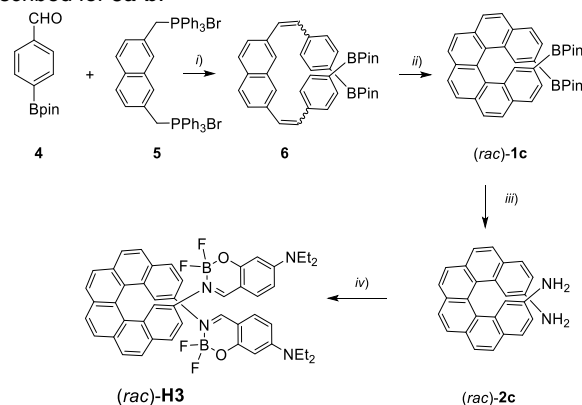
Scheme 2. Synthesis of racemic boranil H3 . i ) n -BuLi, THF, Ar, rt, 3 hrs, 58%; ii ) hν , I 2 , propylene oxide, toluene, Ar, 18 hrs, 57%; iii ) Na 3 , CuSO 4 ·5H 2 O, MeOH, 40°C, 27 hrs, 10% Pd/C, EtOAc rt, 24 hrs, 67%; iv ) 4-(diethylamino)salicylaldehyde, MeOH, reflux, 22 hrs, 98%, then BF 3 ·OEt 2 , DIEA, 1,2-DCE, 85°C, 23 hrs, 91%.
