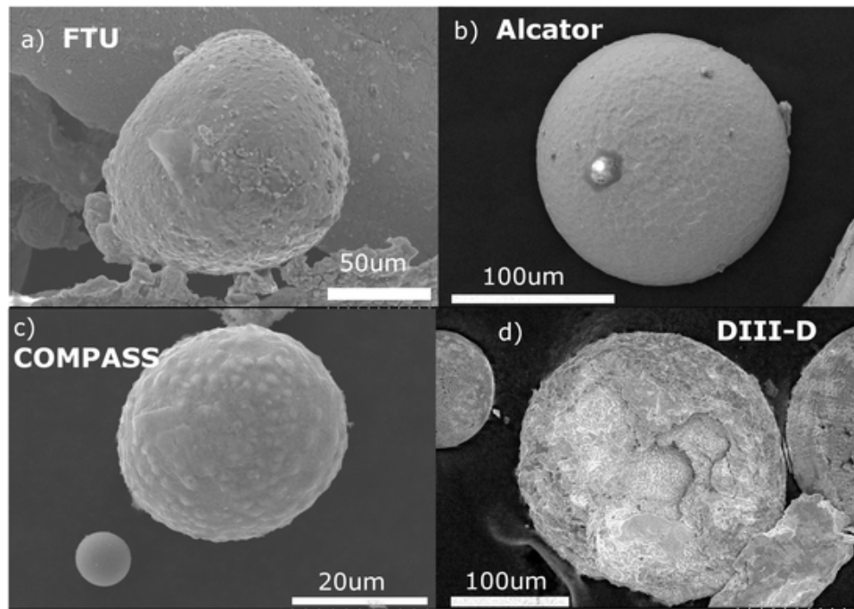
Fig. 5. Spheroidal dust without any clear dendrite-like textured surface and their EDX analysis (at%). (a) SS dust from FTU (C 19.6, O 15.7, Cr 9.6, Fe 47.2, Ni 7.6); (b) SS dust from Alcator (C 0, O 0, Cr 21.2, Fe 70.0 Ni 8.0); (c) SS dust from the COMPASS Co4 batch (C 50.4, O 9.1, Cr 7.9, Fe 27.4, Ni 4.4); (d) SS dust from DIII-D (C 53.4, O 23, Cr 4.7, Fe 15.8, Ni 2.3).
