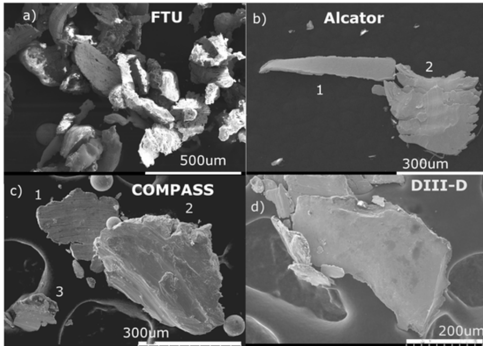
Fig. 1. Dust flakes and their EDX analysis (at%). (a) SS-based dust from FTU (C 3 ± 9, O 15 ± 40, Cr 1 ± 15, Fe 15 ± 53); (b) Ni (1) and SS (2) based dust from Alcator (O 10.1-0, Cr 0-19.6, Fe 0.6-68.5, Ni 88.5-7.7, respectively); (c) SS-based dust from the COMPASS Co3 batch (C 11 ± 33, O 0 ± 5.6, Cr 0.7 ± 16, Fe 45 ± 86, Ni 0 ± 6.6); (d) SS-based dust from DIII-D (C 23.4, O 8.3, Cr 11.3, Fe 46.6, Ni 6.3).
