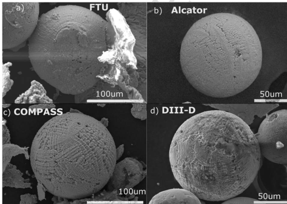
Fig. 4. Spheroidal dust with clear dendrite-like textured surface and their EDX analysis (at%). (a) Ni-based dust from FTU (O 15.4, Cr 12.7, Fe 10.5, Ni 51.24); (b) SS dust from Alcator (O 53.7, Cr 8.0, Fe 32.8, Ni 4.8); (c) SS dust from the COMPASS Co4 batch (O 48.3, Cr 8.7, Fe 32.1, Ni 3.3); (d) SS dust from DIII-D (C 26.9, O 41.6, Cr 7.2, Fe 21.7, Ni 1.9).
