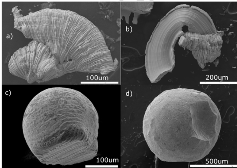
Fig. 2. (a and b) Chips in the Alcator magnetic batch probably due to machining. EDX analysis (at%): O 0.8-2.6, Cr 18.8-19, Fe 69.1-66.3 respectively. (c and d) Spheroidal dust from in-lab Inconel studs welded on SS plates and EDX (at%); (c) magnetic dust (O 63.7, Cr 18.6, Fe 1.4, Ni 0); (d) non-magnetic dust (O 58.7, Cr 28.3, Fe 1.2, Ni 0.5).
