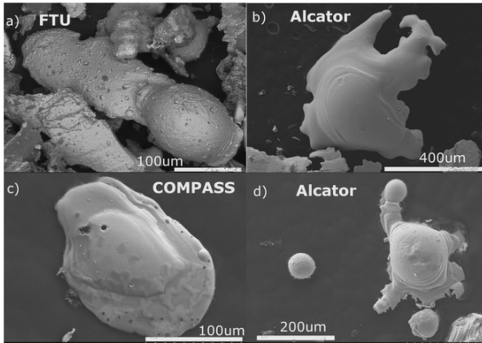
Fig. 3. Dust splashes and their EDX analysis (at%). (a) SS dust from FTU (O 10.1, Cr 14.2, Fe 61.3, Ni 8.0); (b) SS dust from Alcator (O 1.1, Cr 18.8, Fe 72.2, Ni 6.6); (c) Inconel dust from the COMPASS Co2 batch (B 24.6, O 4.8, Cr 14.3, Fe 0.9, Ni 37.7), no splashes in the Co3,4 batches; (d) SS dust from Alcator (O 15.9, Cr 16.3, Fe 51.7, Ni 7.2).
