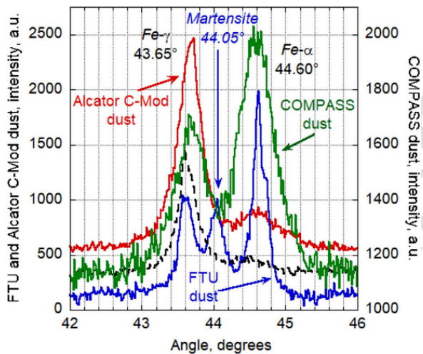
Fig. 6. XRD spectra of the Alcator C-Mod (red), FTU (blue) and COMPASS Co4 (green) magnetic dust batches. The spectrum of untreated AISI316 steel is also shown with the black dashed line. (For interpretation of the references to color in this figure legend, the reader is referred to the web version of this article.)
