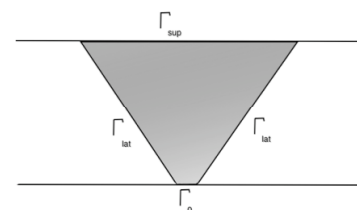
Figure 3 : Geometry of the initial energy director.
