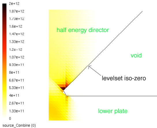
Figure 5 : Source term calculated from the elastic problem for the first time step.
