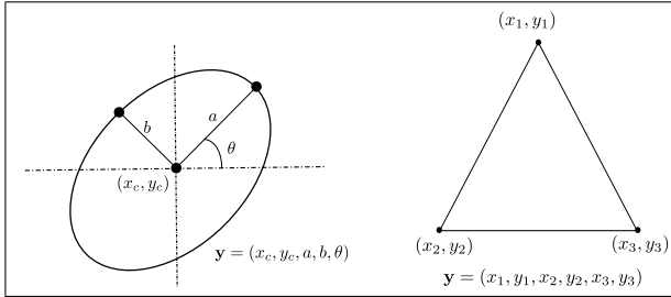
Fig. 3. Output vector representation according to the shape : On the left, ellipses are represented by their center coordinates, major axis and the angle between the major axis and the horizontal axis. On the right, polygons are represented by their vertices coordinates.
