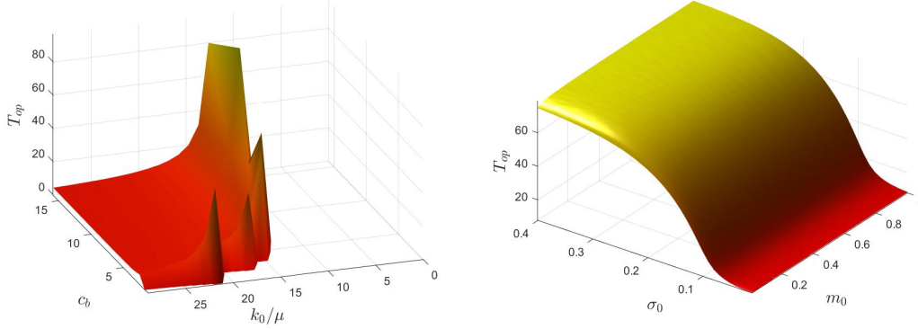
Figure 7: The minimal duration ( T_{\text{op}} ) of drug administration to achieve our TTO objective. (Left) Combined effect of the cost-benefit ratio ( c_b ) and drug activity ( k_0/\mu ), quantified relatively to the host immune response \mu , on the time T_{\text{op}} . (Right) Combined effect of the initial bacterial population size ( m_0 ) and the initial frequency of resistance ( \sigma_0 ) on the time T_{\text{op}} .
