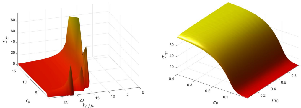
Figure 6: The minimal duration ( T_{\text{op}} ) of drug administration to achieve our TTO objective. (Left) Combined effect of the cost-benefit ratio ( c_b ) and drug activity ( k_0/\mu ), quantified relatively to the host immune response \mu , on the time T_{\text{op}} . (Right) Combined effect of the initial bacterial population size ( m_0 ) and the initial frequency of resistance ( \sigma_0 ) on the time T_{\text{op}} .
