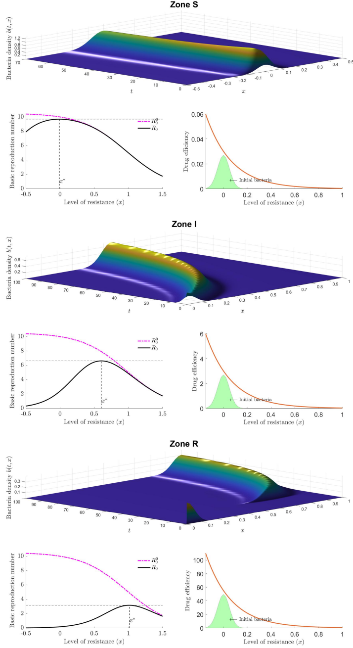
Figure 5: Evolutionary dynamics under sub-inhibitory drug concentrations. (Zone S) sub-lethal dose without emergence of resistance in the bacterial population. (Zone I) sub-lethal dose with emergence of intermediate resistance in the bacterial population. (Zone R) sub-lethal dose with emergence of high resistance in the bacterial population. Parameter values are (\sigma_0, m_0, k_0, p_1/p_0, k_1/k_0) = (0.05, 0.05, 0.03, 0.5, 0.01) , (0.05, 0.05, 3, 0.5, 0.01) , (0.05, 0.05, 55, 0.5, 0.01) for zones S, I, and R respectively. Other parameters are shown by Table 1.
