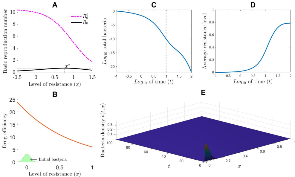
Figure 4: Evolutionary dynamics with lethal treatment. Parameter values are (\sigma_0, m_0, k_0, p_1/p_0, k_1/k_0) = (0.05, 0.05, 20, 0.5, 0.3) or default as shown in Table 1. The vertical dashed line in panel (C) shows the time from which the total bacterial population is always \leq 10^{-10} .
