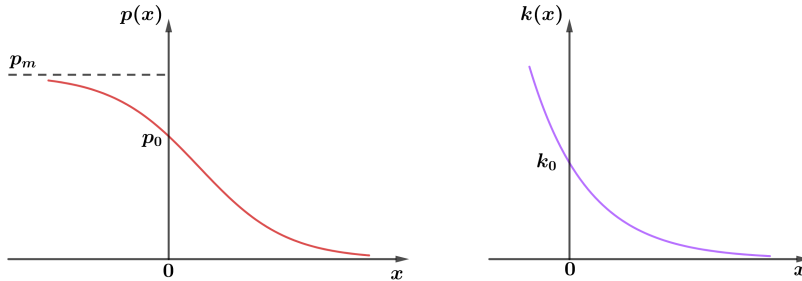
Figure 1: (Left) Intrinsic growth rate p(x) of bacterial population with a level of resistance x \in \mathbb{R} . (Rigth) Drug activity k(x) on bacterial population with resistance level x \in \mathbb{R} .
