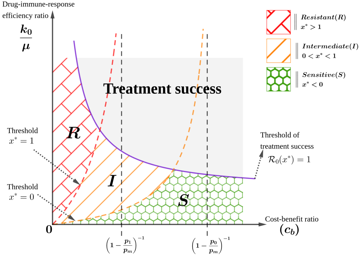
Figure 3: Evolutionary resistance level ( x^* ) with respect to the resistance's cost-benefit ratio ( \log(\Delta)/\log(1 + \theta) ) and drug efficiency ( k_0/\mu ) on the reference sensitive strain, quantified relatively to the host immune response ( \mu ). Areas R , I , and S correspond to parameter combinations where the evolutionary level of resistance x^* is such that x^* \geq 1 , 0 < x^* < 1 , and x^* \leq 0 respectively. The treatment success holds above the level set \{\mathcal{R}_0(x^*) = 1\} , that is, for the zone in gray. The treatment is unsuccessful below the level set \{\mathcal{R}_0(x^*) = 1\} , that is, for zones R , I and S (below the purple curve). The curves labelled ' x^* = 0 ' (in yellow) and ' x^* = 1 ' (in red) indicate 'sensitive' and 'resistant' thresholds.
