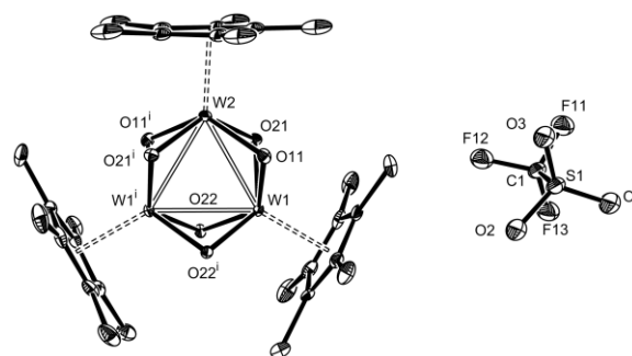
Figure 3. A view of the relative orientation of cation and anion in the structure of [Cp* 3 W 3 O 6 ](CF 3 SO 3 ), 2. Only one of the two symmetry-related orientations of the trifluoromethylsulfonate anion and of the Cp*(2) ligand are shown for the sake of clarity.
