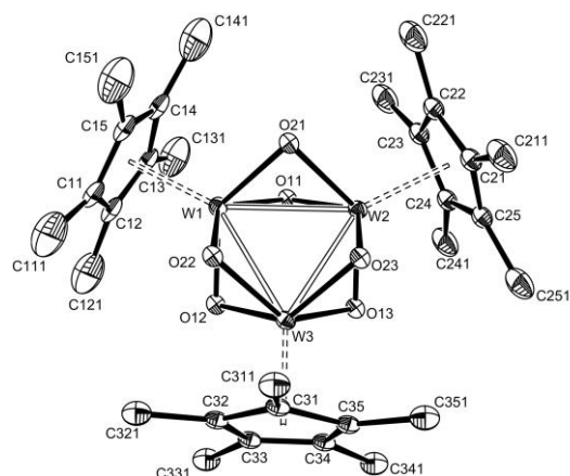
Figure 7. An ORTEP view of the [\text{Cp}^*_3\text{W}_3\text{O}_6]^+ ion from the structure of compound 3 .
