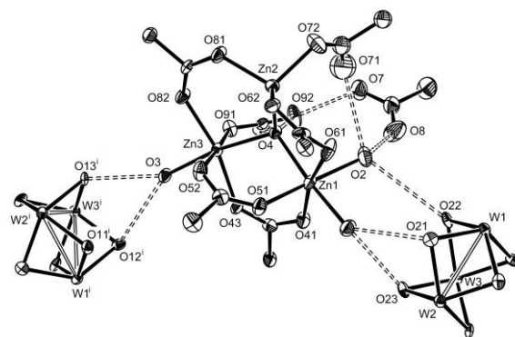
Figure 5. A view of the arrangement between the [\text{Zn}_3(\mu_3\text{-O})(\mu\text{-CF}_3\text{COO})_4(\text{CF}_3\text{COO})(\text{CF}_3\text{COOH})(\text{H}_2\text{O})_3]^- anion, the interstitial \text{CF}_3\text{COOH} molecule, and the [\text{Cp}^*\text{W}_3\text{O}_6]^+ cation in compound 3 . The cation \text{Cp}^* ligands and the aqua H atoms have been removed and only the coordination spheres of the Zn atoms are shown for clarity [Symmetry code: (i) \frac{1}{2}+x , \frac{3}{2}-y , z-\frac{1}{2} ].
