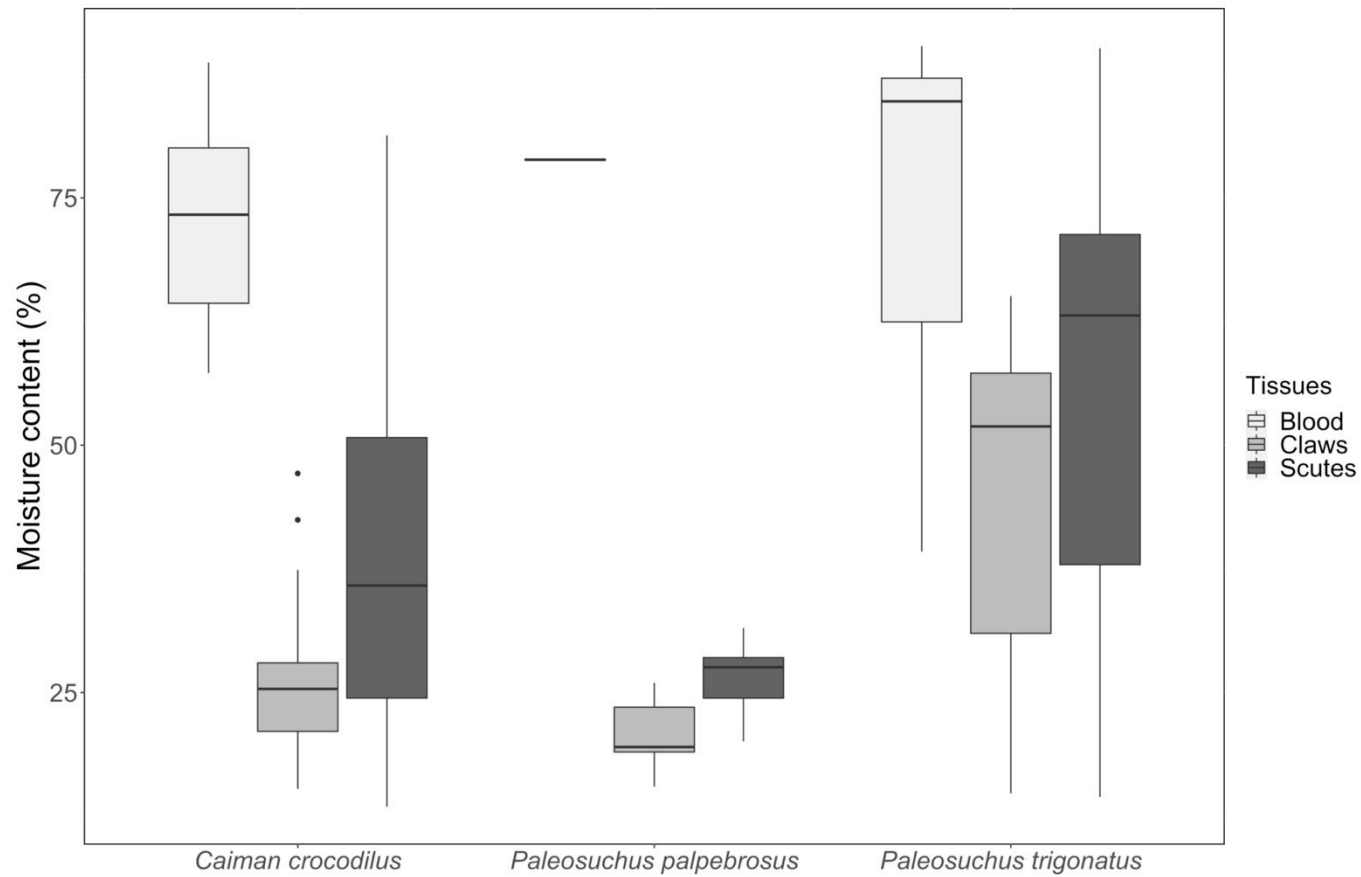
Figure 2. Moisture content measured in total blood, claws and scutes (%) of spectacled caiman, Caiman crocodilus , dwarf caiman, Paleosuchus palpebrosus , and smooth-fronted caiman, Paleosuchus trigonatus , in French Guiana. The top and bottom of the boxes represent the first and last quartiles, the line across the box represents the median, the whiskers represent the fifth and ninety-fifth percentiles, and the circles represent outliers.
