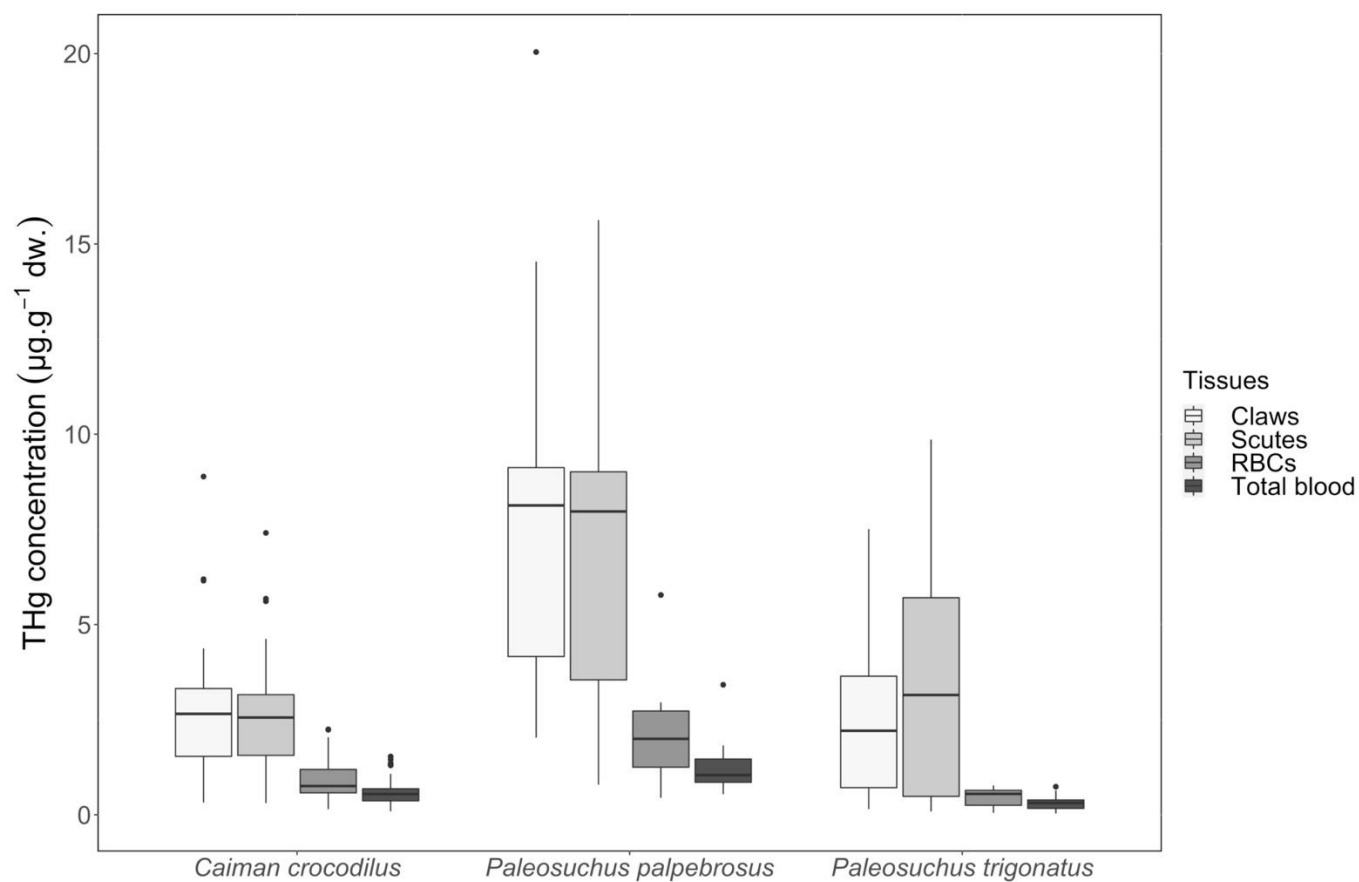
Figure 5. THg concentrations measured in claws, scutes, red blood cells (RBCs) and total blood ( \mu\text{g.g}^{-1} dw) of spectacled caiman, Caiman crocodilus , dwarf caiman, Paleosuchus palpebrosus and smooth-fronted caiman, Paleosuchus trigonatus , in French Guiana. The top and bottom of the boxes represent the first and last quartiles, the line across the box represents the median, the whiskers represent the fifth and ninety-fifth percentiles, and the circles represent outlier.
