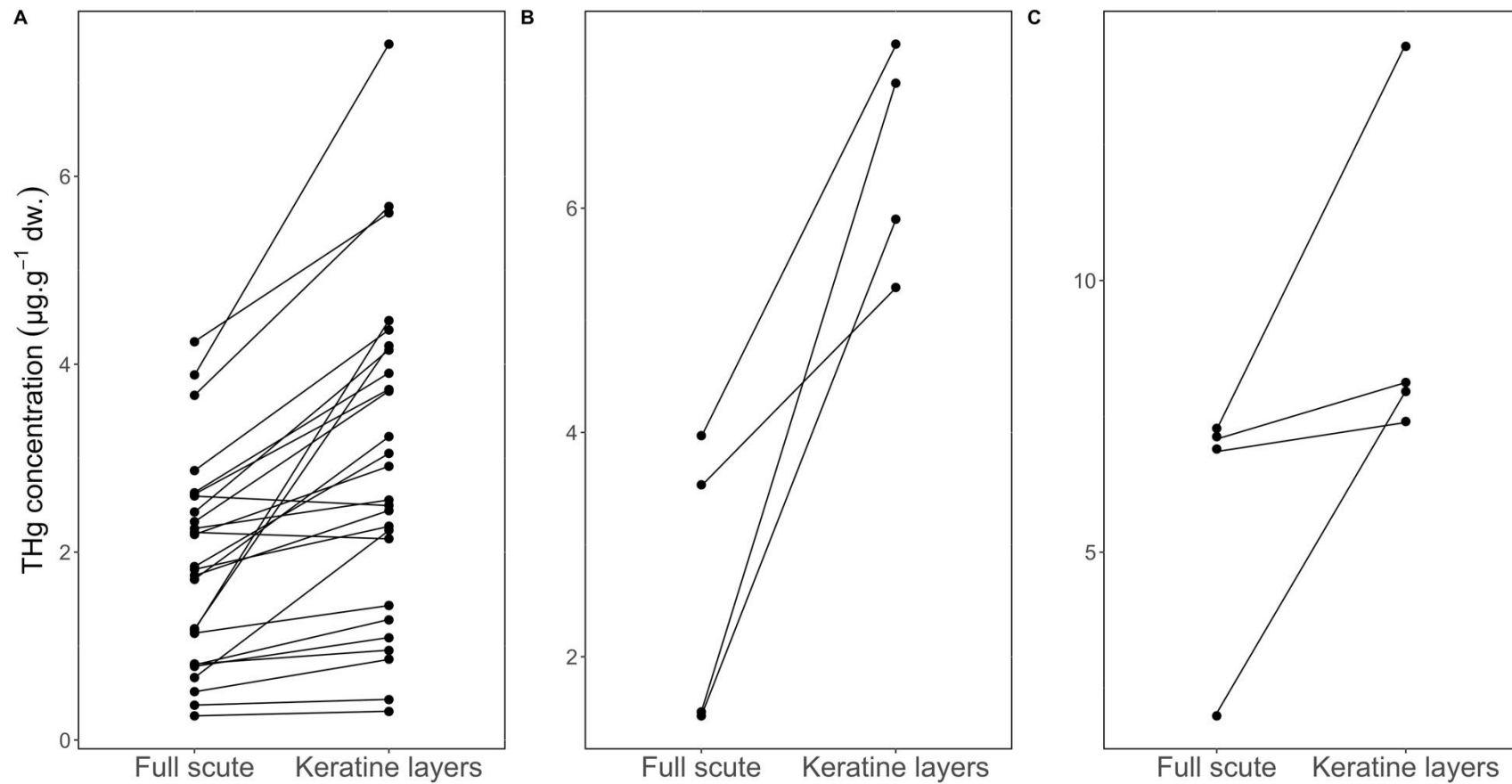
Figure 3. THg concentrations measured in full scutes and scute keratin layers ( \mu\text{g.g}^{-1} dw.) of spectacled caiman, Caiman crocodilus (A: n = 26 , paired t-test: t = -5.44 , p < 0.001 ), smooth-fronted caiman, Paleosuchus trigonatus (B: n = 4 , paired t-test: t = -4.71 , p = 0.02 ) and dwarf caiman, Paleosuchus palpebrosus (C: n = 4 , paired t-test: t = -2.18 , p = 0.12 ), in French Guiana. Each pair of connected dots correspond to one individual.
