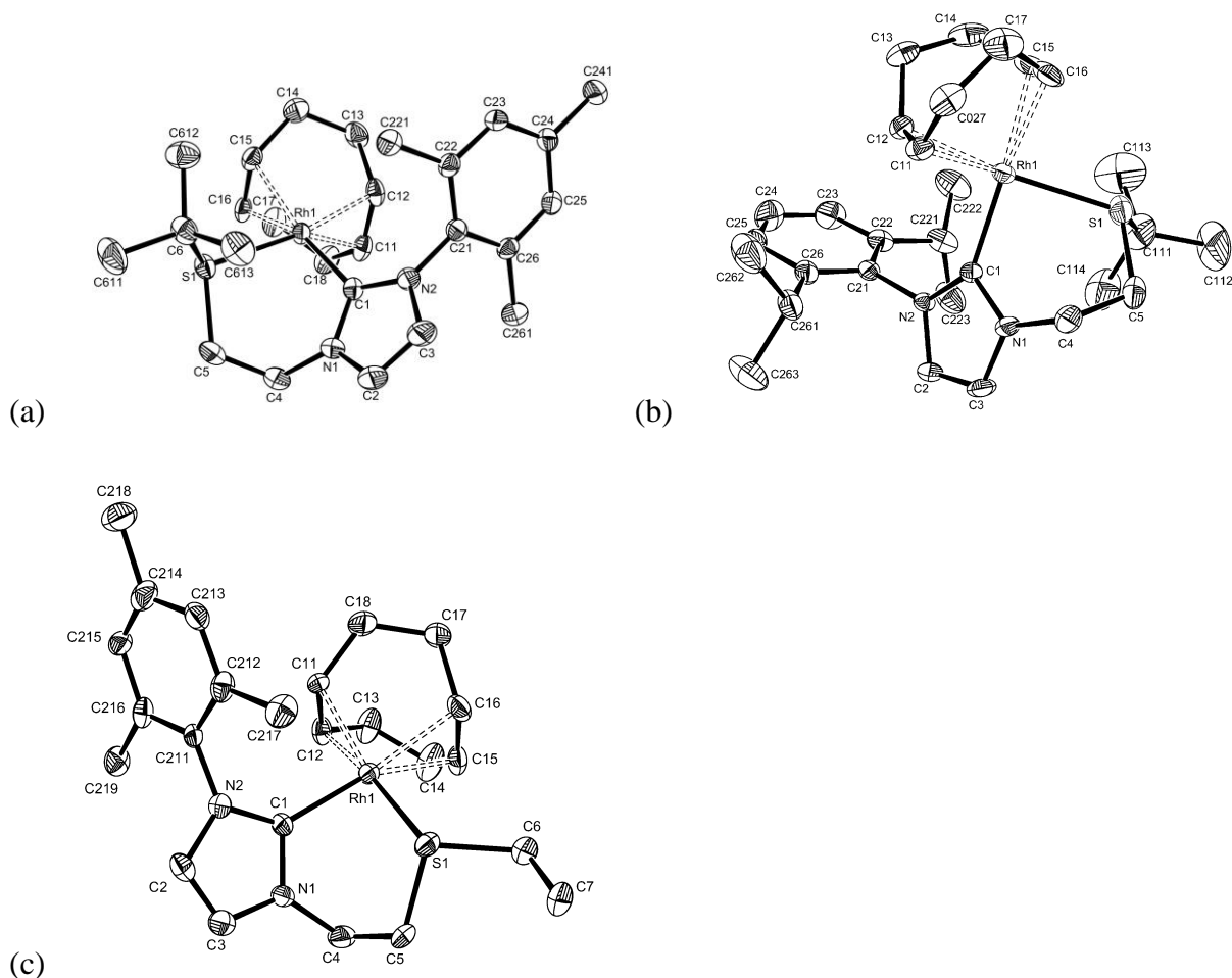
Figure 5 ORTEP views of the cations in complexes 18 (a), 19 (b) and 20 (c). Ellipsoids are represented at the 30% probability level. Hydrogen atoms, the counter ion ( \text{BF}_4 ) and a co-crystallized \text{CDCl}_3 molecule ( 18 ) are omitted for clarity.
