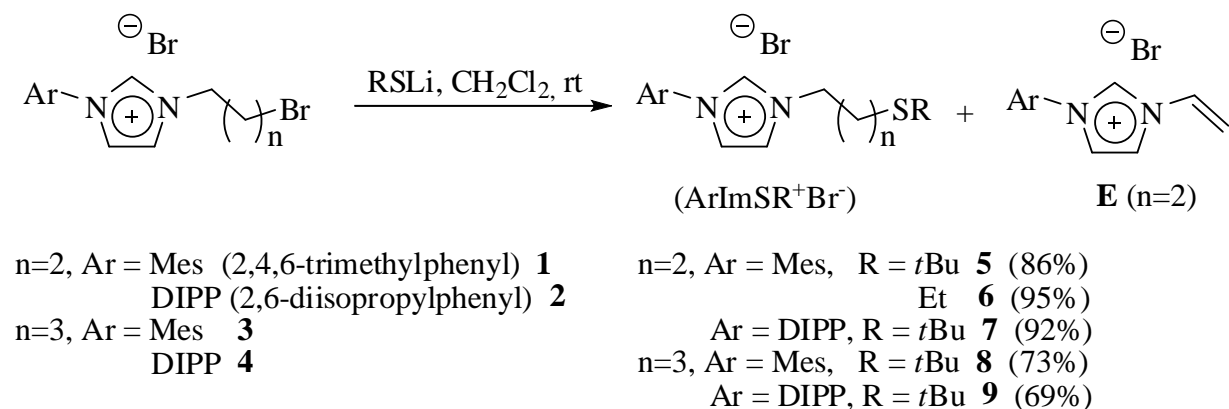
Scheme 1 Nucleophilic substitution on 1-4 bromides by lithium alkylthiolate reagents.
