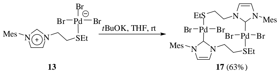
Scheme 3 Palladium(II) complexes synthesis.
