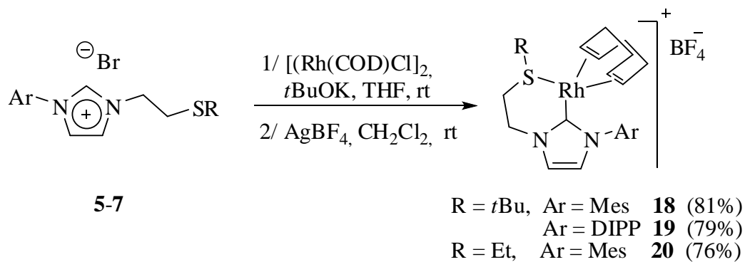
Scheme 4 Rhodium(I) complexes synthesis.
