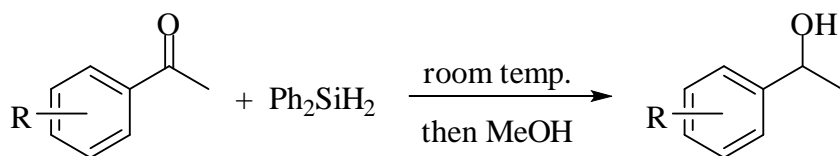
Scheme 5 Hydrosilylation of acetophenone and its derivatives with Rh I complexes.
