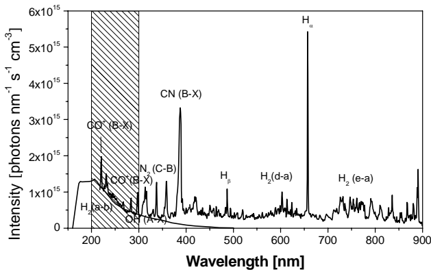
Figure 3. H 2 spectrum with fitted H 2 (a-b) continuum
