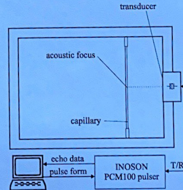
Fig. 4. Experimental setup (top view).
