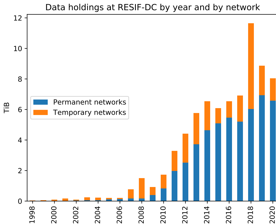
Figure 6: Current validated data holdings at Résif-DC grouped by year. This figure illustrates the growth of the data produced by seismological networks since 1998.
