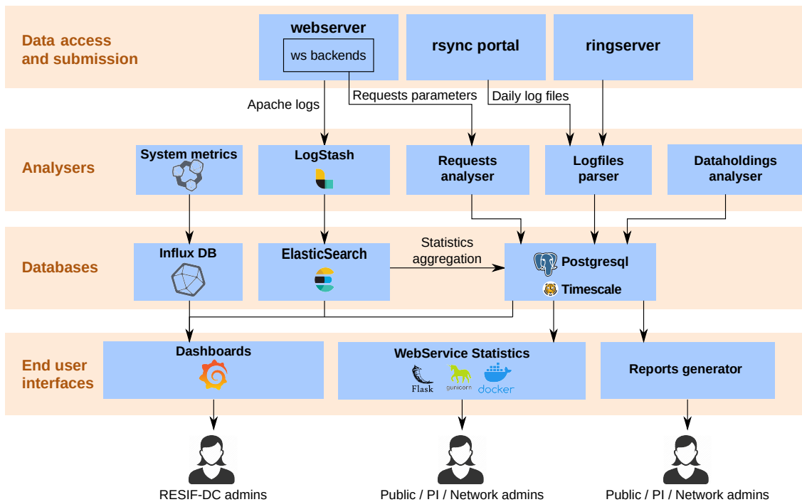
Figure 8: The logging system analyzes events from heterogeneous sources (e.g., web access logs, webservices requests, server logs); the statistics are computed by different analyzers and aggregated in one central database (Postgresql). The statistics can be queried by various interfaces intended for different audiences; in particular a public webservice resifws-statistics is available.
