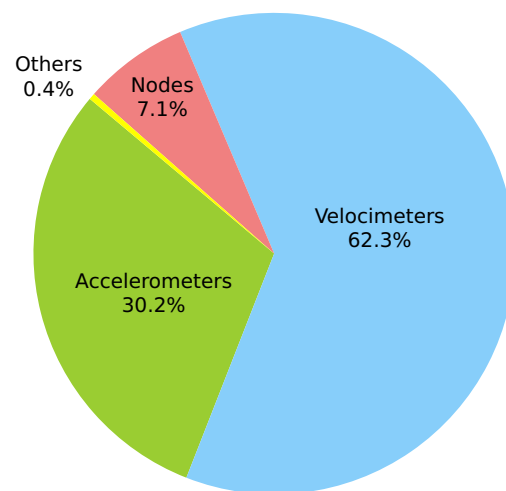
Figure 3: Distribution of data volumes in Résif archive, as of January 1st, 2021. Velocimetric data represents 62.3%. Accelerometric data represents 30.2%, Data from very short period "node" geophones represents 7.1% and other data, like meteorological time series, accounts for 0.4%.
