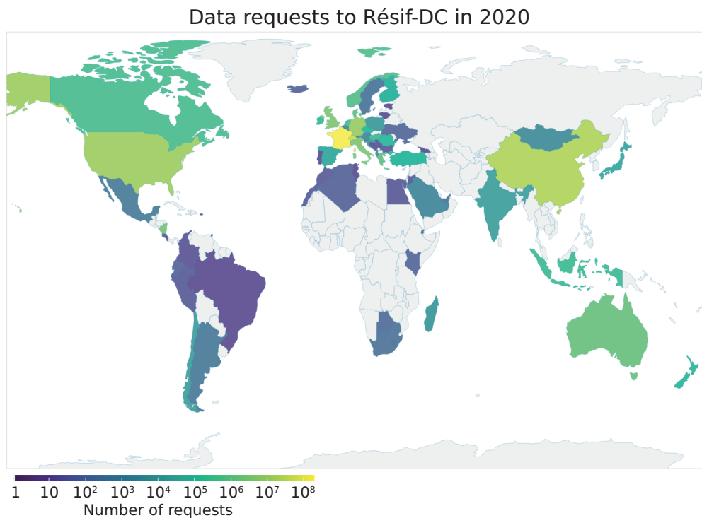
Figure 10: Geographical distribution of data requests to Résif-DC in 2020.
