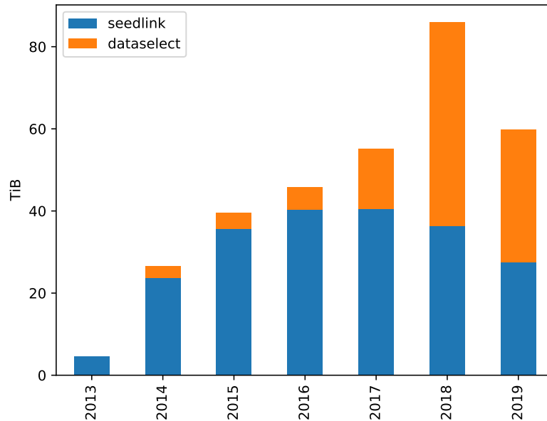
Figure 7: Amount of waveform data distributed yearly through SeedLink (real-time) and FDSN datasetselect. Note that statistics from the now retired EIDA Arclink services are not included.
