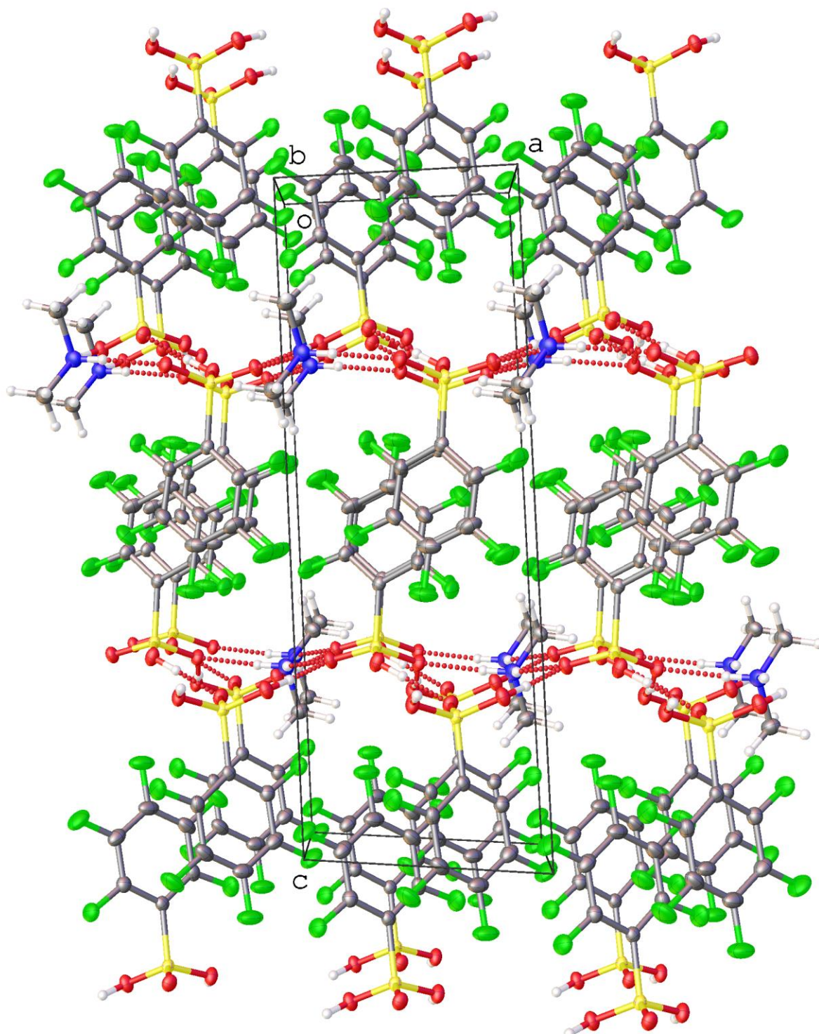
Figure 8. View along b of 4,4'\text{-DMA}^+ showing a single-layer stacking motif.
