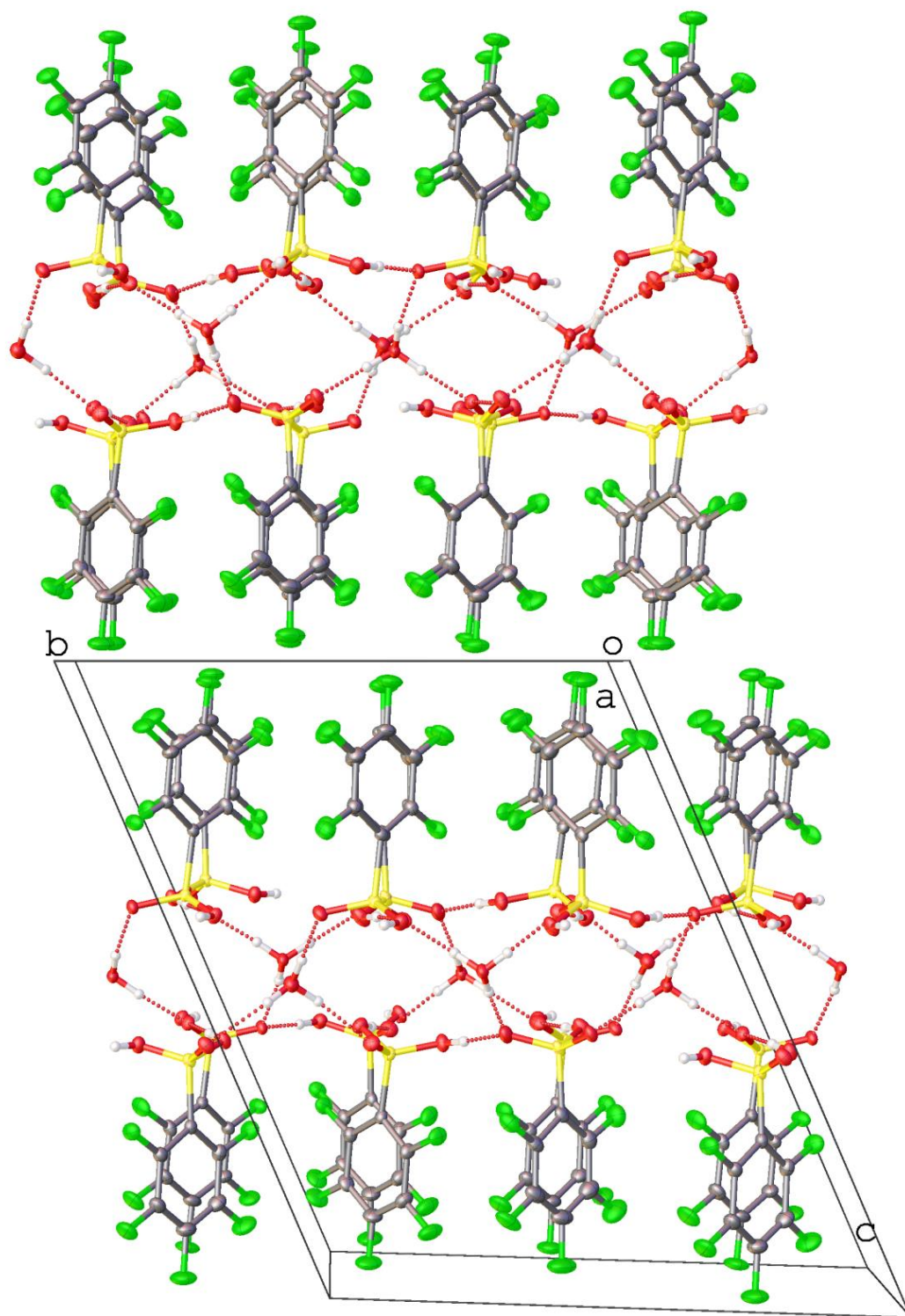
Figure 2. View along a of 4.4 · H 3 O + showing a bilayer stacking motif.
