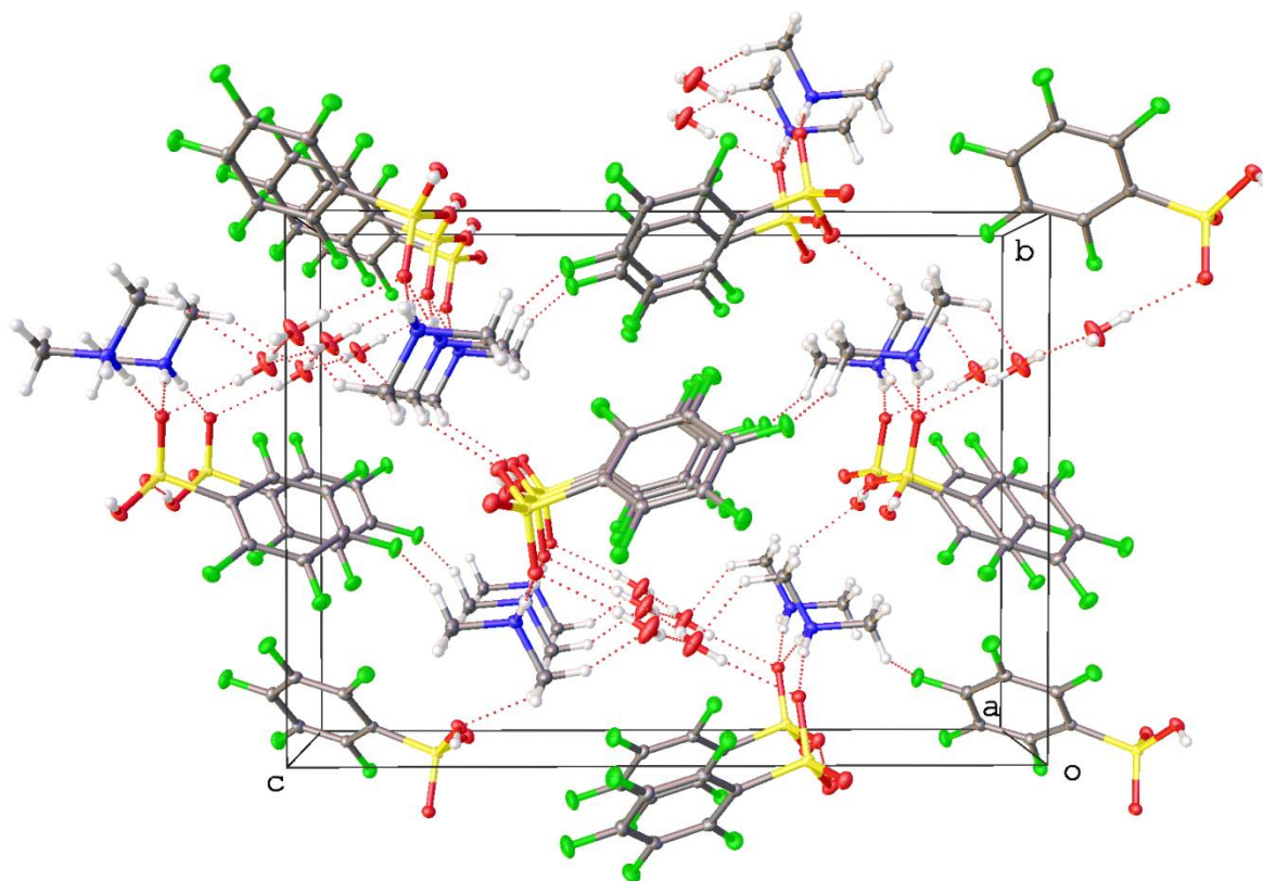
Figure 7. View along a of 4 - .DMA + .H 2 O showing a single-layer stacking motif.
