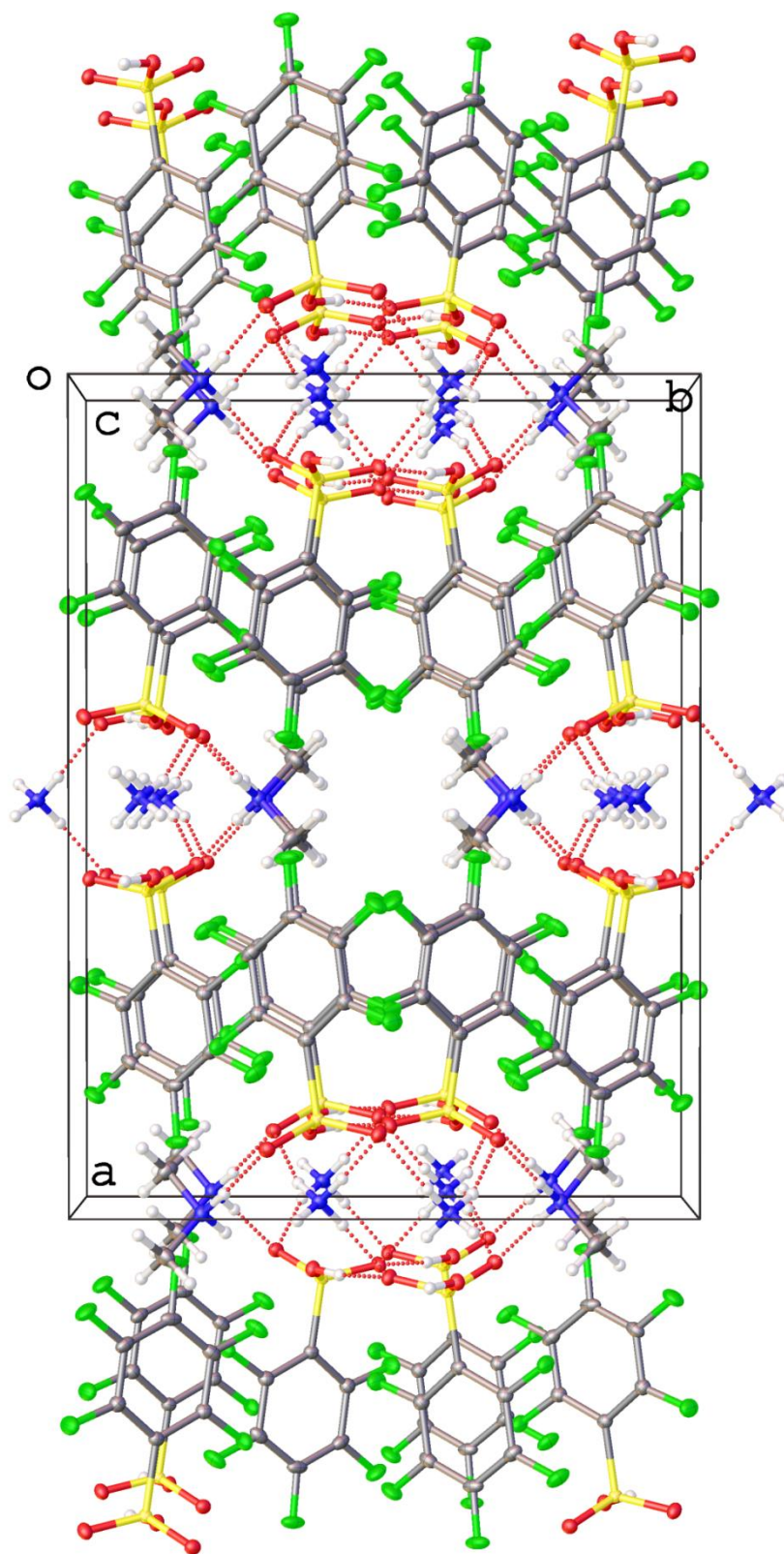
Figure 9. View along c of 4^{\cdot-}.\text{DMA}^+.\text{NH}_4^+ showing a single-layer stacking motif.
