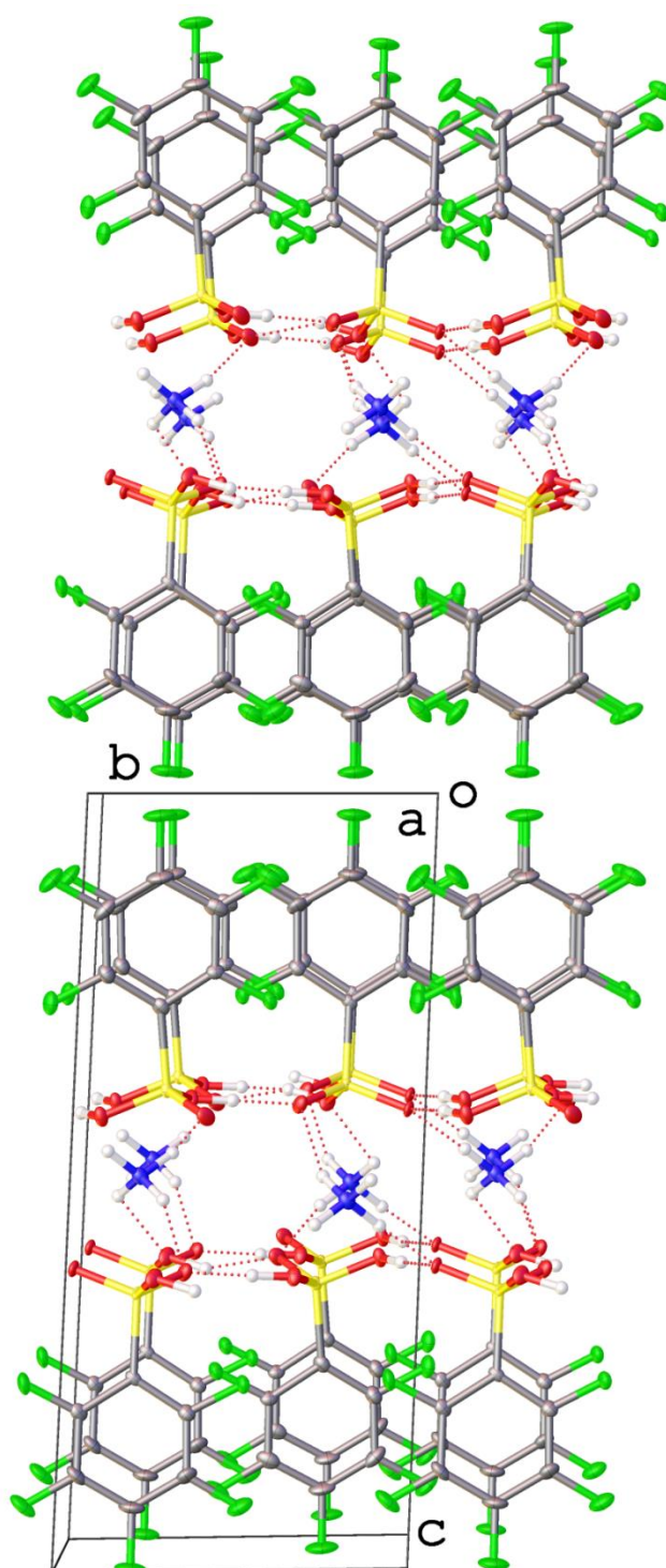
Figure 5. View along a of 4.4^-\cdot\text{NH}_4^+ showing a bilayer stacking motif.
