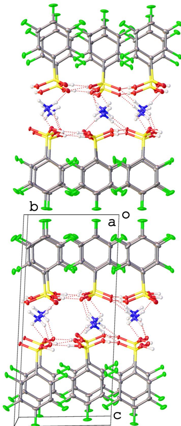
Figure 5. View along a of 4\cdot\text{DMA}^+\cdot\text{NH}_4^+ showing a bilayer stacking motif.
