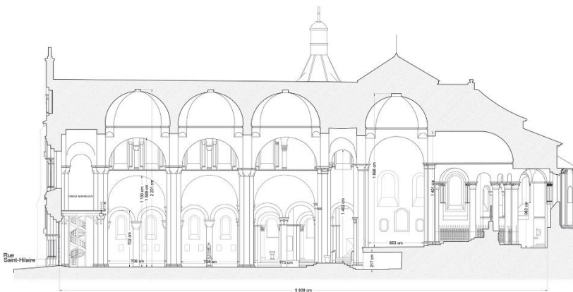
Figure 10: Longitudinal section extracted from a 3D mesh – The church “Saint Hilaire le Grand” church , Poitiers (France) – Archeovision Prod
