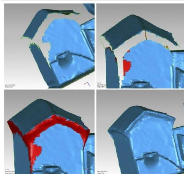
Figure 5: Point cloud hole filling- Nantes project F.Laroche/Epotec LS2N
