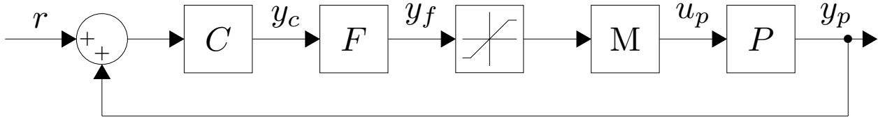
Figure 1: General view of control allocation problem.
