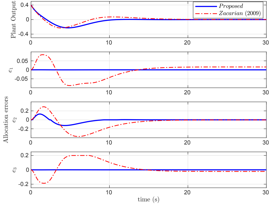
Figure 4: Example 2: Output and allocation errors for both the proposed strategy and [14].
