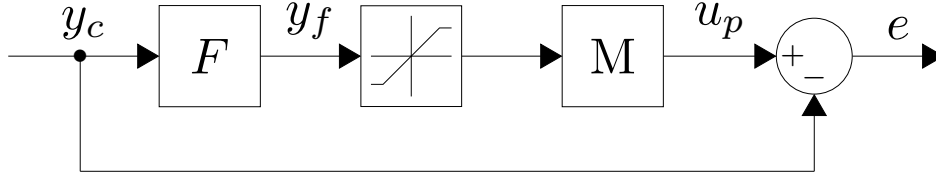
Figure 2: Diagram illustrating mapping from y_c to allocator error e .
