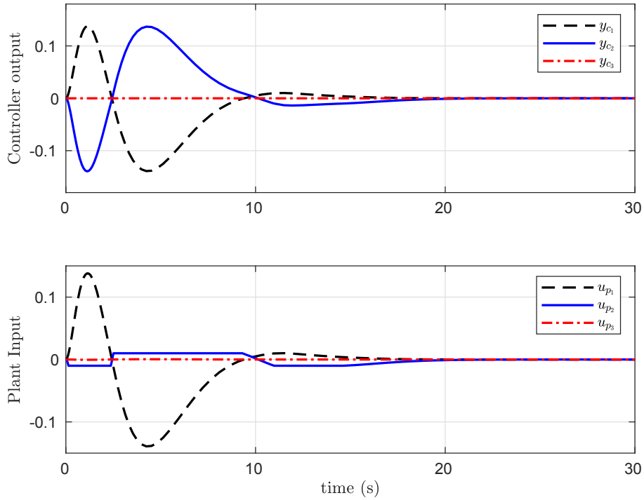
Figure 5: Example 2: Controller output and plant input signals for the proposed strategy.
