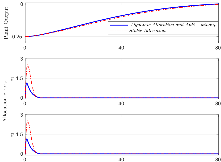
Figure 3: Example 1: Output and allocation errors.
