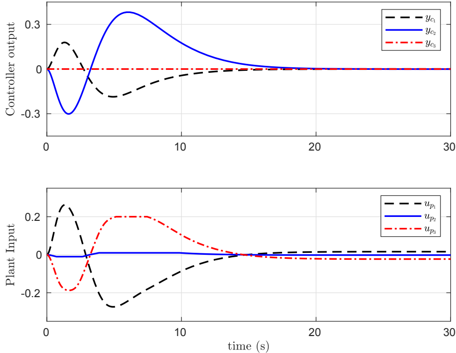
Figure 6: Example 2: Controller output and plant input signals for the strategy from [14].
