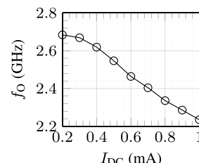
Fig 4 (a) Measured output frequency spectra in dependence of I_{DC} for H = 1 \text{ kOe} . (b) Measured MTJ-based STO's output power P_{out} and (c) centre oscillation frequency f_0 in dependence of injected DC current I_{DC}
