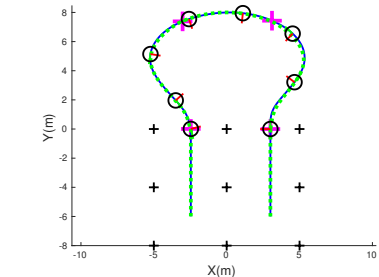
(c) Dashed: Reference path - Solid: Robot trajectory - Pink crosses: controller switches - Black crosses: trees
