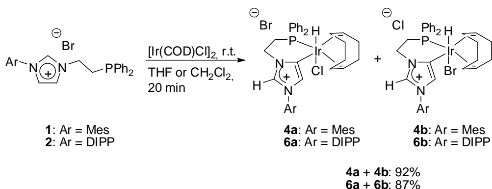
Scheme 2. Mixture of isomers 4a + 4b from the reaction of ligand 1 , or isomers 6a + 6b from the reaction of ligand 2 , with [Ir(COD)(μ-Cl)] 2 .
