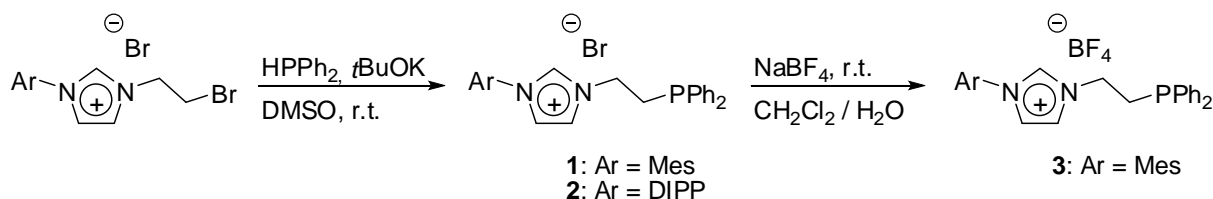
29 30 Scheme 1. Synthesis of phosphine-imidazolium salts. Mes = mesityl or 2,4,6- 31 trimethylphenyl; DIPP = 2,6-diisopropylphenyl.
