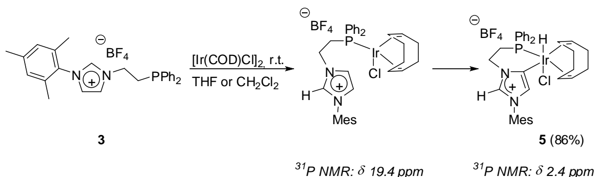
Scheme 3. Synthesis of complex 5 via an iridium(I) intermediate.
