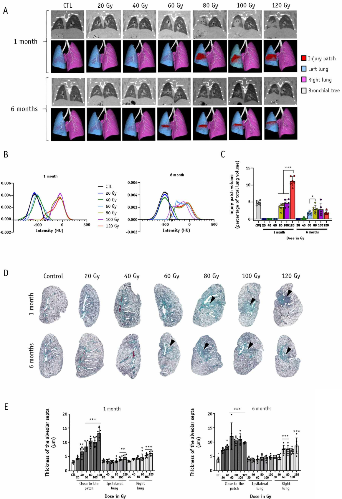
Fig. 5. Dose effect of left lung arc therapy. (A) Representative micro-computed tomography images and 3-dimensional reconstructions in controls and 1 and 6 months after exposure to 20, 40, 60, 80, 100, or 120 Gy. Different colors have been used to differentiate the injury patch (red), the left lung (blue), the right lung (pink), and the main bronchi (white). (B)
