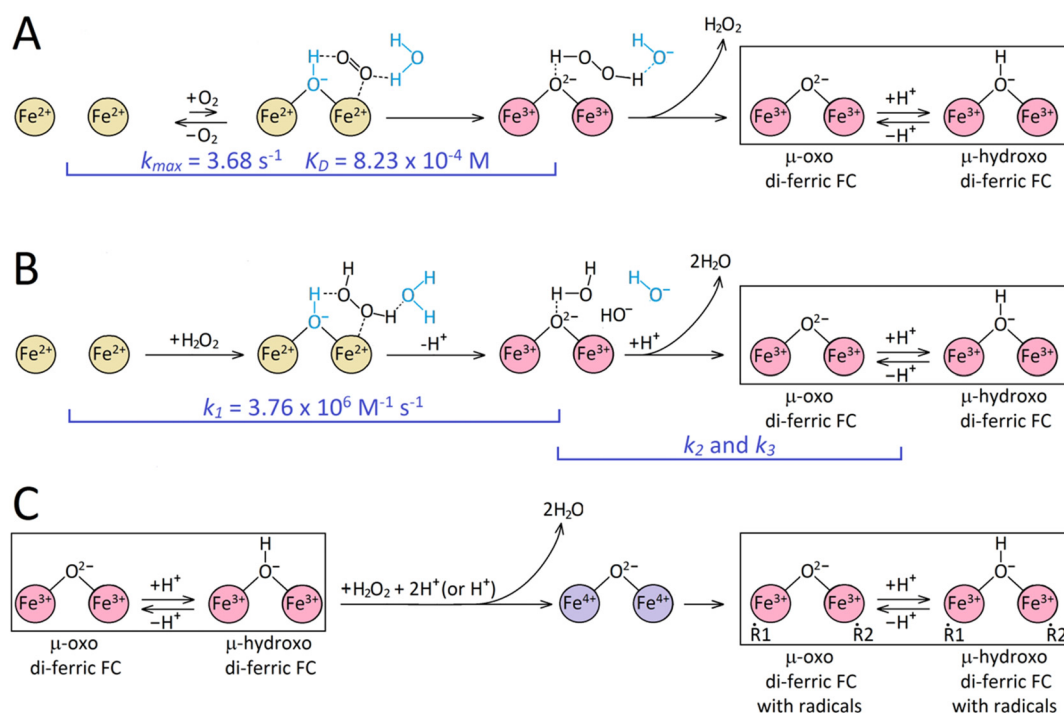
Figure 8. The three sets of reactions of iron oxidation at the FC of Ecbfr—by \text{O}_2 (A), by \text{H}_2\text{O}_2 (B) and the reaction of the oxidized (di-ferric) FC with \text{H}_2\text{O}_2 (C) leading to free radical formation. We put forward the hypothesis that both \text{O}_2 and \text{H}_2\text{O}_2 bind to one of the two iron atoms which must be facilitated by structural water and/or hydroxyls (shown in blue color) or a nearby residue(s), such as Glu94, that provide hydrogen bonding to \text{O}_2 and \text{H}_2\text{O}_2 .
